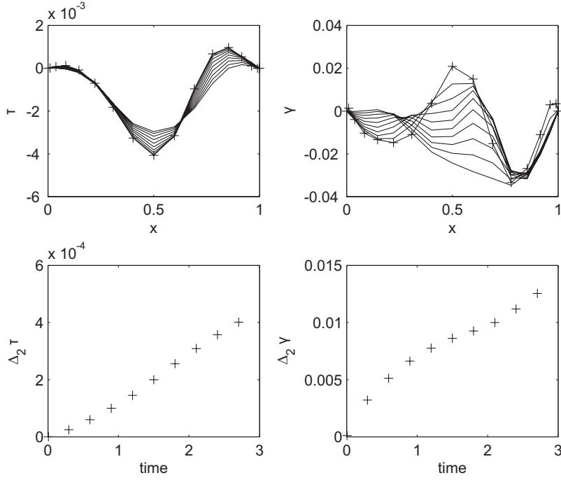
Figure 12: Same as Fig. 11, but for the quartic RNS simulation of the lid-driven cavity flow.
