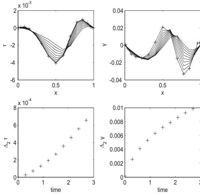
Figure 11: Errors in the cubic RNS simulation of the lid-driven cavity flow. The (absolute) errors \Delta\tau and \Delta\gamma are shown as functions of the location for different times; the L_2 -errors \Delta_2\tau and \Delta_2\gamma are shown as functions of the nondimensionalized time.
