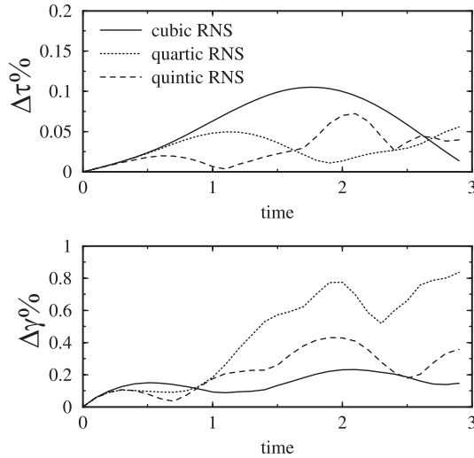
Figure 2: RNS simulations for \tau and \gamma in the perturbed channel flow with \epsilon = 10^{-3} . The percentage error for \tau is obtained as \Delta\tau\% = \frac{100}{N} \left[ \sum_{i=1}^N |\tau - \tau_i| \right] / \max_i |\tau_i| where \tau_1, \dots, \tau_N are the \tau values at N gridpoints x_1, \dots, x_N \in [0, 1] ; the definition of \Delta\gamma\% is similar.
