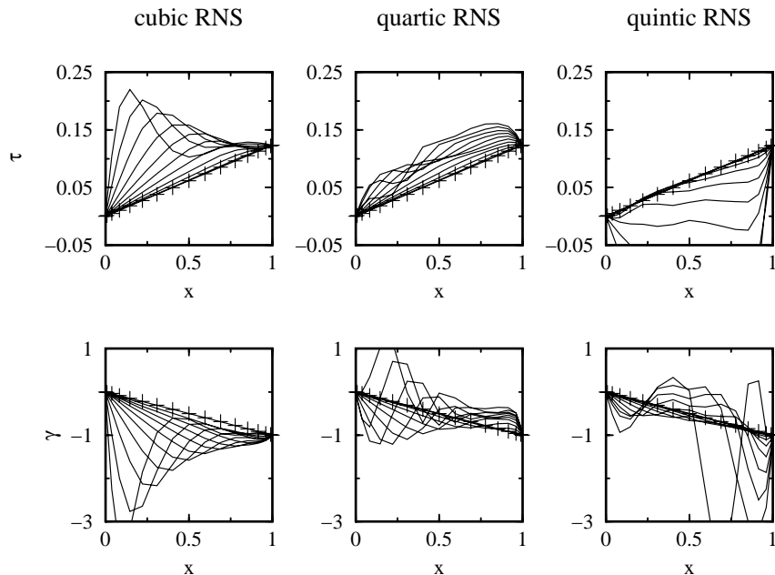
Figure 7: Evolution of the \tau and \gamma profiles in the cubic, quartic, and quintic RNS equations for the viscous stagnation point flow. The snapshots are taken with nondimensional time step \Delta \bar{t} = 0.1 ; the final simulation time is \bar{t} = 1.5 . Crosses mark the exact solution.
