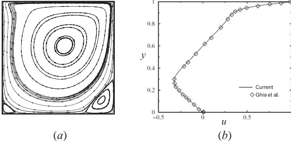
Figure 10: (a) Streamlines at the steady state of a lid-driven cavity flow at Re = 400 . (b) Comparison of a u -velocity profile along the midplane for the steady state of a lid-driven cavity at Re = 400 .
