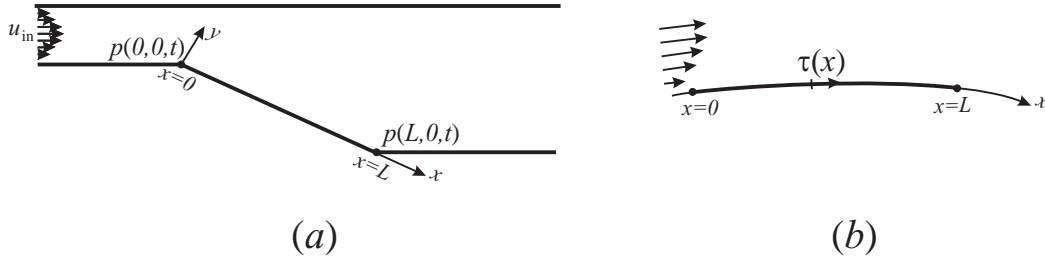
Figure 1: Possible domains of definition for the RNS equations in flow control problems. (a) Inclined wall section of a two-dimensional diffuser (b) Wall section of a two-dimensional streamlined body.
