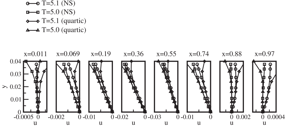
Figure 15: Same as Fig. 14, but for the quartic RNS simulation.
