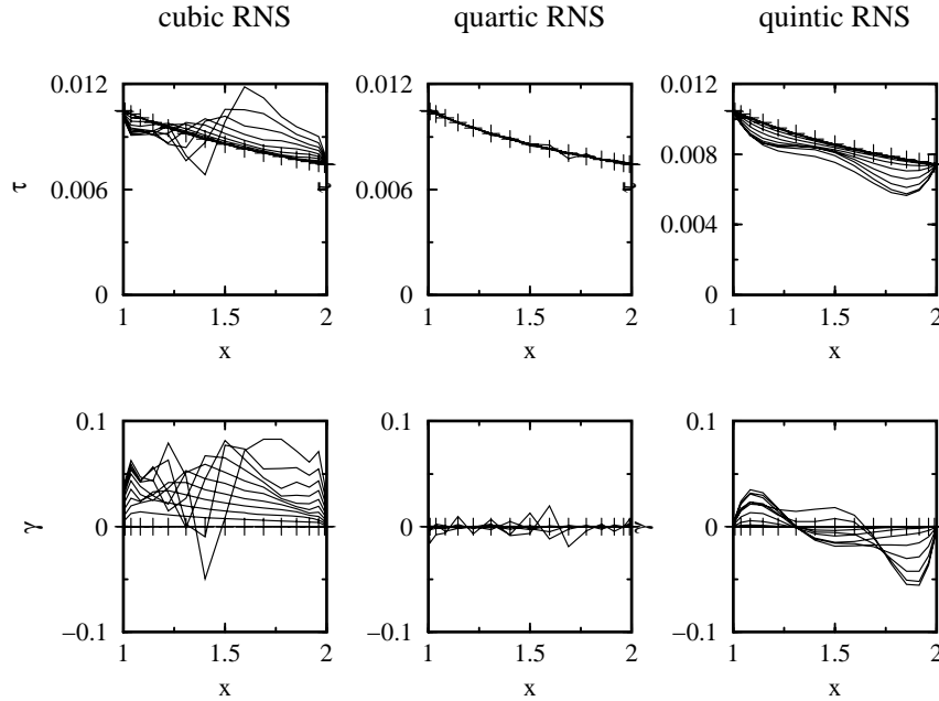
Figure 5: Evolution of the \tau and \gamma profiles in the cubic, quartic, and quintic RNS equations for the Blasius boundary layer flow. The snapshots are taken with nondimensional time step \Delta\bar{t} = 0.3 ; the final simulation time is \bar{t} = 3 . Crosses mark the exact solution.
