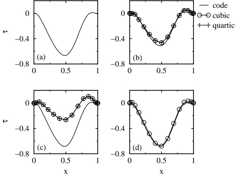
Figure 13: Comparison of skin-friction values predicted by a Navier-Stokes simulation (“code”), and by the cubic and quartic RNS simulation for the initial unsteady phase of the lid-driven cavity flow at \text{Re} = 400 . (a) Initial condition at \bar{t} = 5.0 (b) Simulation at \bar{t} = 5.1 (c) simulation at \bar{t} = 5.2 (d) Same as (c) but with initial conditions re-initialized at \bar{t} = 5.1 .
