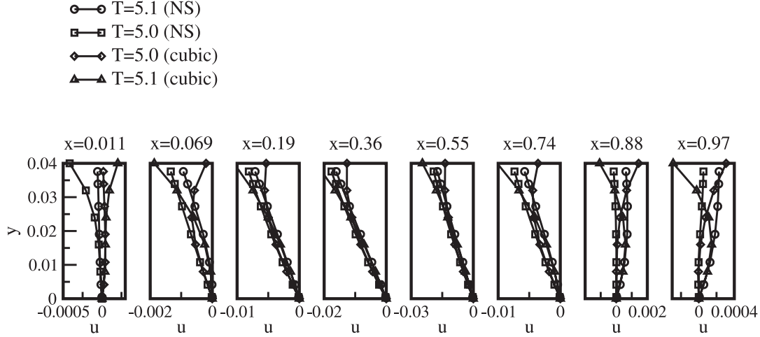
Figure 14: The u -component of the lid-driven cavity velocity field at \bar{t} = 5.0 and \bar{t} = 5.1 at different locations near the y = 0 boundary. “NS” refers to Navier-Stokes simulations; “cubic” refers to cubic RNS simulations.
