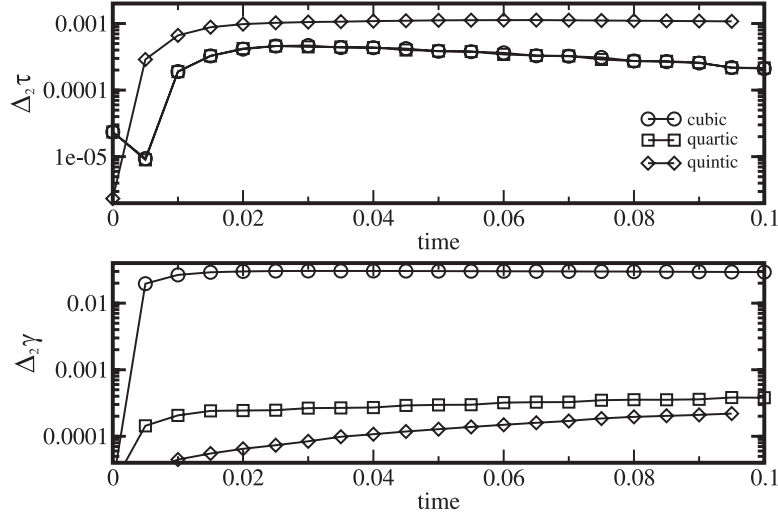
Figure 8: L_2 error in \tau and \gamma as a function of time for flow oscillating over an infinite plate.
