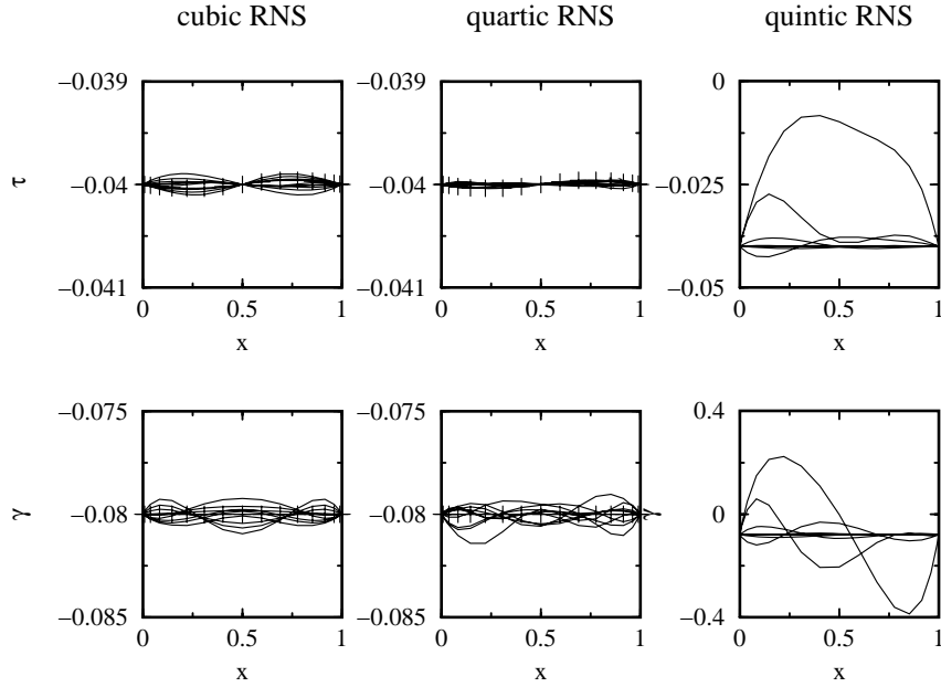
Figure 3: Evolution of the \tau and \gamma profiles in the cubic, quartic, and quintic RNS equations for the channel flow. The snapshots are taken with nondimensional time step \Delta\bar{t} = 0.1 ; the final simulation time is \bar{t} = 10 for the cubic and quartic RNS equations, and \bar{t} = 7 for the quintic RNS equation. Crosses mark the exact solution.
