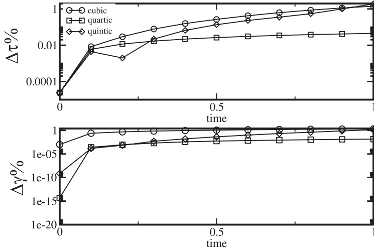
Figure 4: Percentage of error in \tau and \gamma as a function of time for the Blasius profile.
