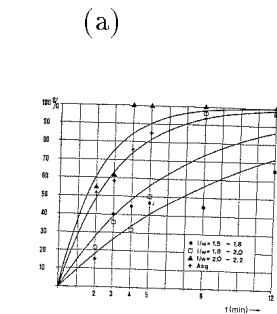
Figure 1. Recovery of different fractions in the top of the jighead. The relation between the time, during which the various fractions go to the top of the bed and the 1/y-ratio has not been quantified. It is however clear that if the 1/y-ratio increases, the separation of the top becomes more difficult or for a high recovery of SIC more impossible, for this reason the recovery has to be low for a high grade SIC product, with increasing jig time more SIC will move to the top, because in the last step of the desizing process the separation will take place based on the difference in shape of the particles.
