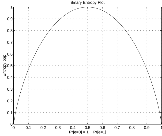
Figure 11: Plot of entropy for a binary signal as a function of sample probability
