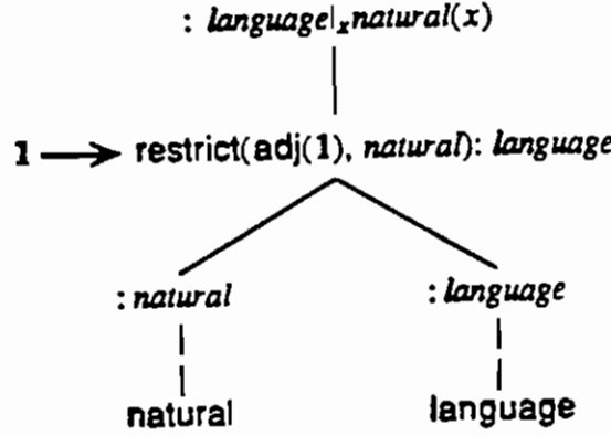
Figure 8: Adjectival Modification
