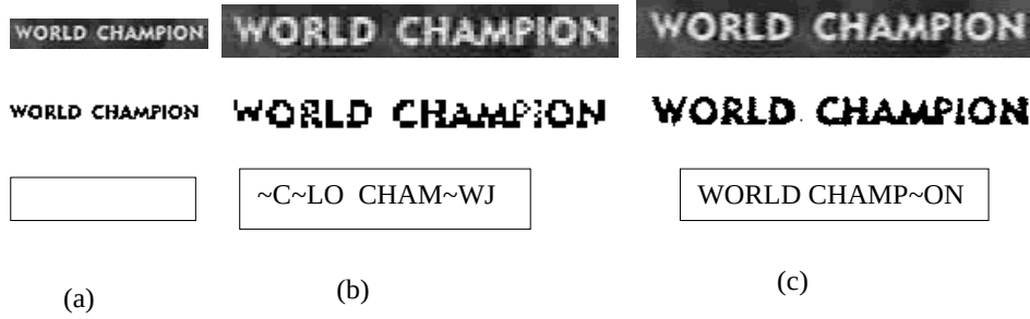
Figure 25: Comparison of OCR results. (a)No enhancement, (b)Zero-order interpolation, (c)Shannon interpolation.
