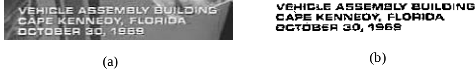
Figure 24: (a) A text block with a font size of approximately 6-7 pixels, (b) Binarization by manually picking the best threshold. There is no output from commercial OCR software although the text is clearly readable.
