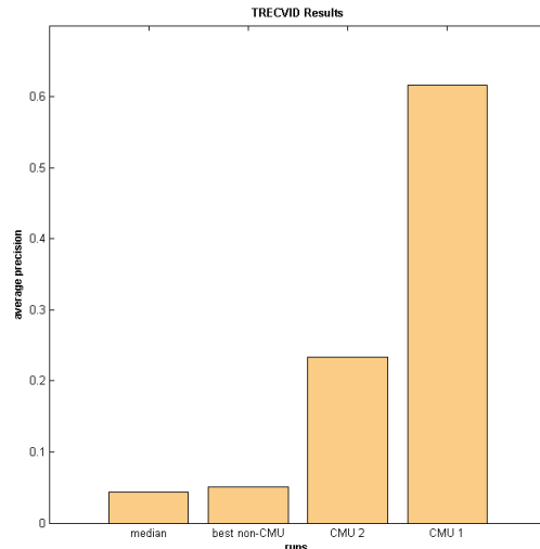
Figure 5: TRECVID 2003 results for news subject monologue detection. The first column, labelled median, indicates the median average precision for all submitted runs. The second column, labelled best non-CMU, is the score of the second best system. The third column, labelled CMU 2, shows our performance based on the common annotation. The fourth column, labelled CMU 1, shows our best submitted run.
