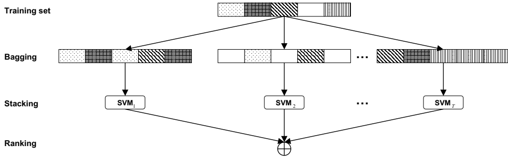
Figure 4: Classifier ensemble architecture.
