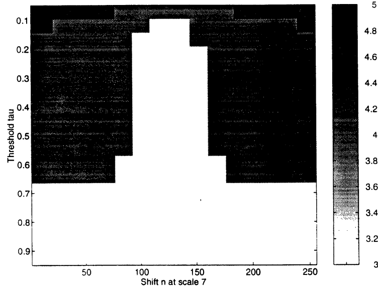
Figure 14: Space-varying optimal scale of reconstruction as a function of \tau . The horizontal axis represents the shift n at the finest scale, M_g = 7 , the vertical axis is the value of \tau , and the grey tones represent the finest scale of resolution supported by the data at shift n using threshold \tau . Darker colors indicate finer scales.
