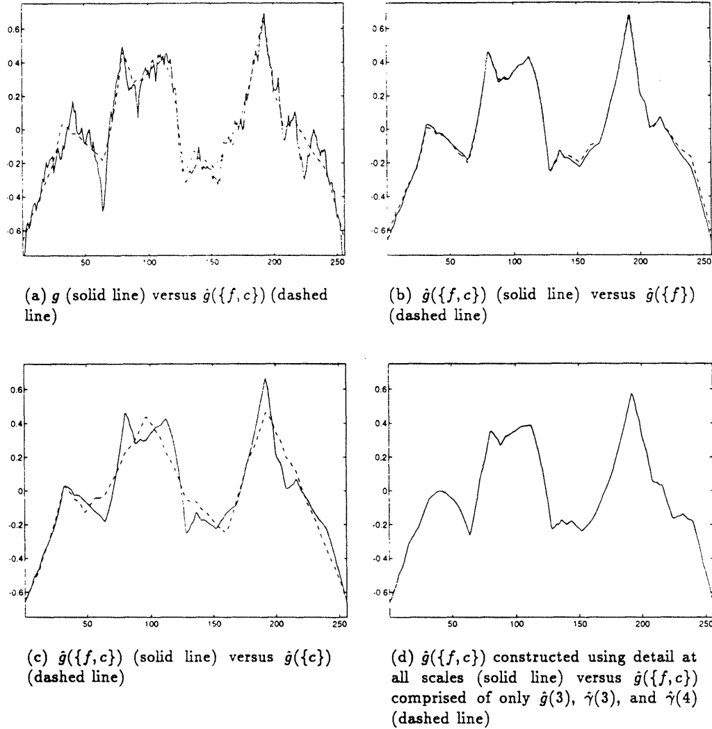
Figure 7: Estimates of g using various combinations of fine and coarse scale data for the equal SNR experiment. From (b) and (c) we observe that given both sets of equally noisy data, the estimator uses primarily the information from the process y_f . In (d), g is reconstructed ignoring any detail estimates, \hat{\gamma}(m) , at scales finer than 4 and compared to the estimate \hat{g} in which all available detail is used. In this case we observe that y_f and y_c provide little useful information at scales 5 through 7.
