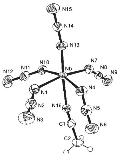
Figure 2. ORTEP plot of [\text{Nb}(\text{N}_3)_5(\text{CH}_3\text{CN})] . Thermal ellipsoids are shown at the 50% probability level. Selected bond lengths [Å] and angles [°]: Nb–N1 2.031(3), Nb–N4 1.998(3), Nb–N7 2.004(3), Nb–N10 2.017(3), Nb–N13 1.935(3), Nb–N16 2.259(3), N1–N2 1.217(4), N2–N3 1.139(4), N4–N5 1.212(4), N5–N6 1.133(4), N7–N8 1.212(4), N8–N9 1.129(4), N10–N11 1.211(4), N11–N12 1.132(4), N13–N14 1.205(4), N14–N15 1.137(4), N16–C1 1.139(4), C1–C2 1.447(5); N1–Nb–N4 87.55(12), N1–Nb–N7 165.51(11), N1–Nb–N10 82.89(12), N1–Nb–N13 99.16(12), N1–Nb–N16 84.59(10), N4–Nb–N7 93.90(12), N4–Nb–N10 162.91(12), N4–Nb–N13 96.38(12), N4–Nb–N16 81.15(10), N7–Nb–N10 91.93(11), N7–Nb–N13 95.01(12), N7–Nb–N16 81.40(11), N10–Nb–N13 99.11(12), N10–Nb–N16 83.86(10), N13–Nb–N16 175.45(11), Nb–N1–N2 132.7(2), Nb–N4–N5 141.9(2), Nb–N7–N8 144.1(2), Nb–N10–N11 132.3(2), Nb–N13–N14 168.8(3), Nb–N16–C1 170.6(3).
