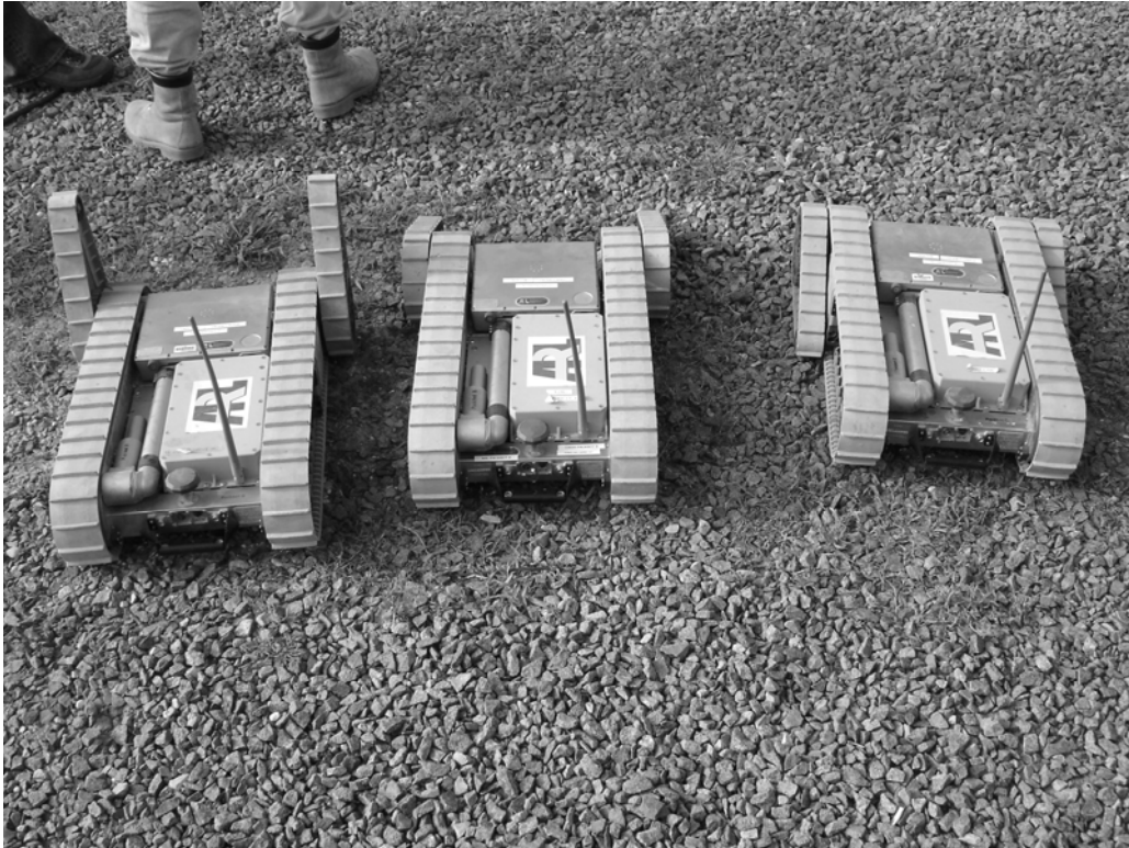
Figure 3. PackBots showing ARL ad hoc payloads.
