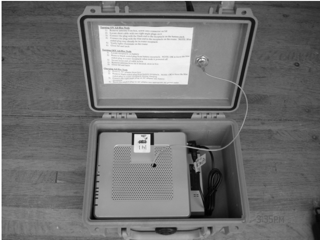
Figure 4. Internals of ARL ad hoc drop-off node.
