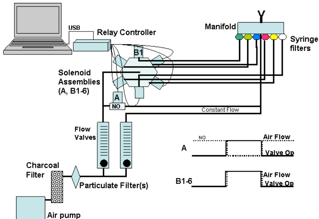
Fig 7: Schematic of the Lorig olfactometer that will be used in this study. The olfactometer is designed to exhibit no change of air velocity while switching between samples ( http://psych.wlu.edu/cnl/olfactometer_construction.htm ).
