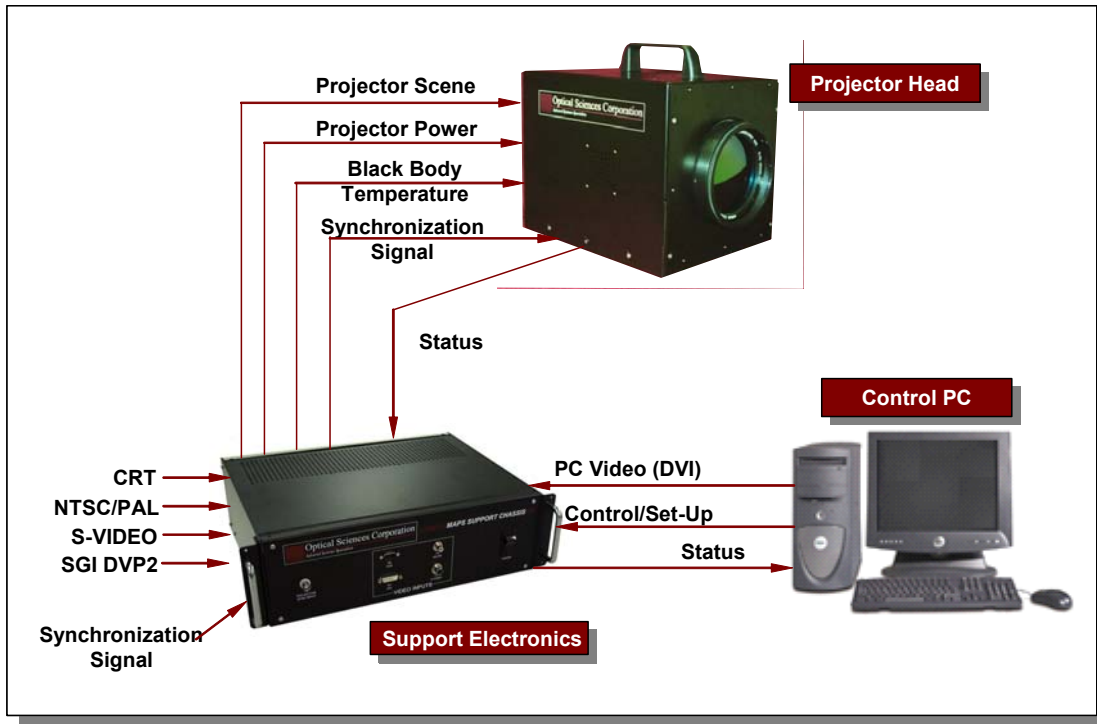
Figure 4: MAPS Block Diagram
