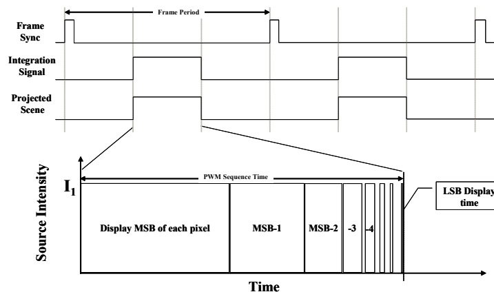
Figure 7: Synchronized PWM Timing
