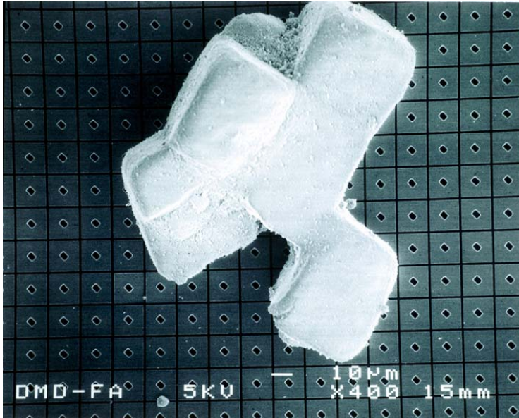
Figure 2: DMD with Grain of Salt on Surface
