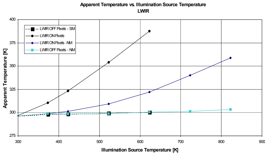
Figure 18: LWIR Apparent Temperature vs. Illumination Source Temperature
