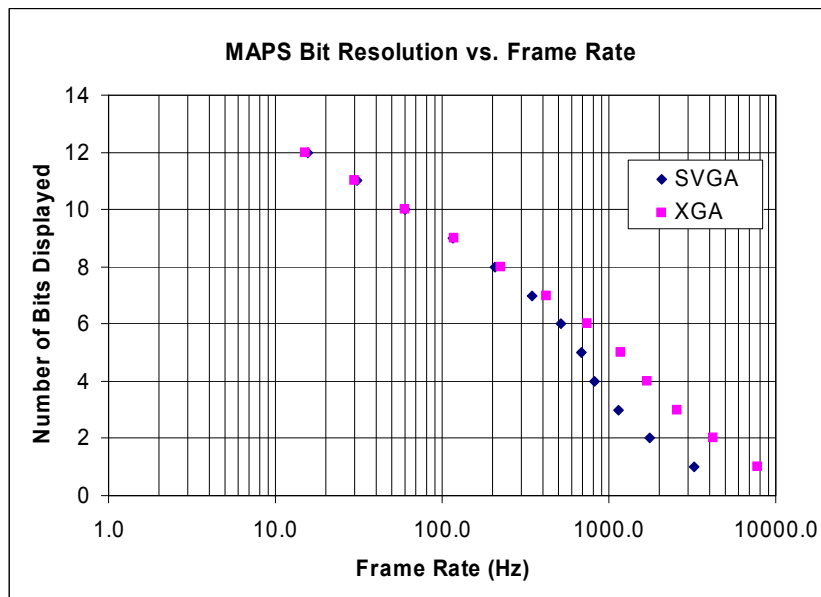
Figure 9: MAPS Bit Resolution vs. Frame Rate for Single DMD
