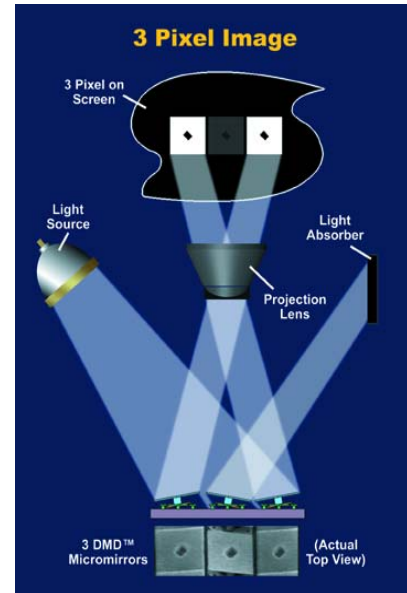
Figure 3: DMD Illumination
