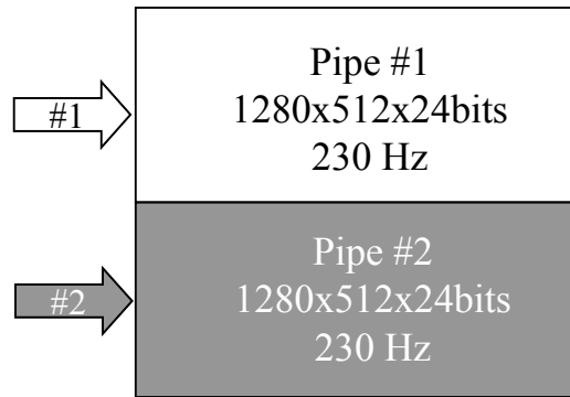
Figure 15: SXGA Two-Pipe Video Architecture
