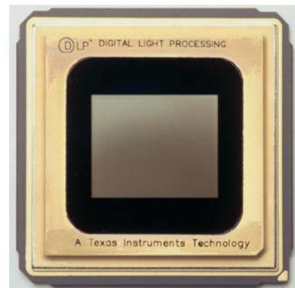
Figure 1: DMD Package
