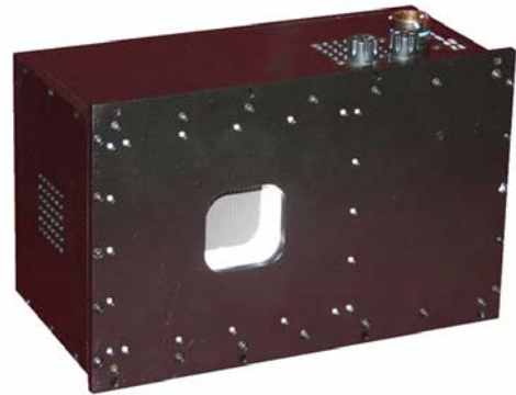
Figure 16: High Temperature Blackbody
