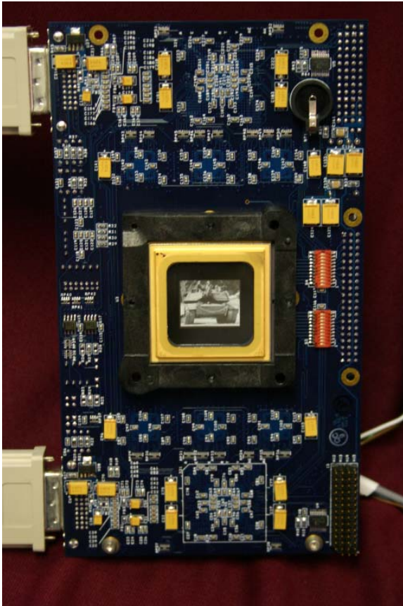
Figure 13: SXGA Drive Electronics & DMD
