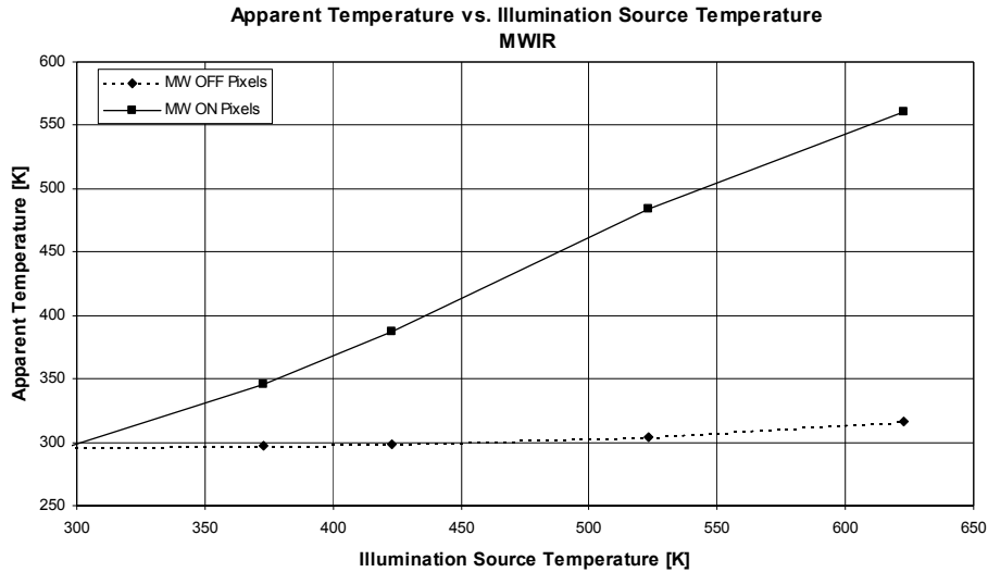
Figure 17: MWIR Apparent Temperature vs. Illumination Source Temperature
