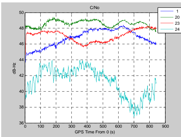
Figure 19 Satellite C/No
