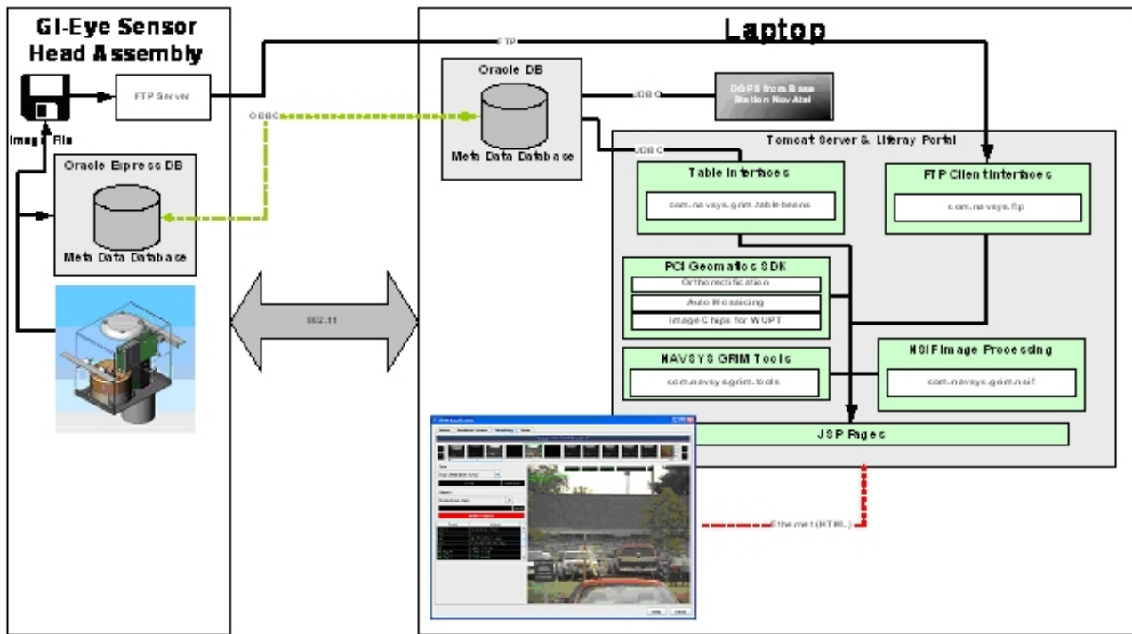
Figure 8 GI-Eye and GRIM Architecture
