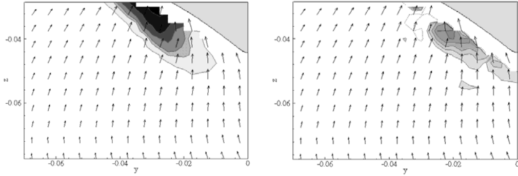
Figs. 25a and 25b: longitudinal velocity iso-levels and cross-flow vectors ( left ), longitudinal vorticity and cross-flow vectors ( right ); section 0.8 (port-side view).
