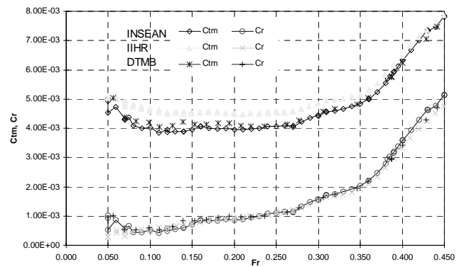
Fig. 5: Comparison for C_{TM} and C_R obtained by INSEAN (model 2340, \lambda = 24.8 ), IIHR (model 5512, \lambda = 46.6 ), DTMB (model 5415, \lambda = 24.8 ).
