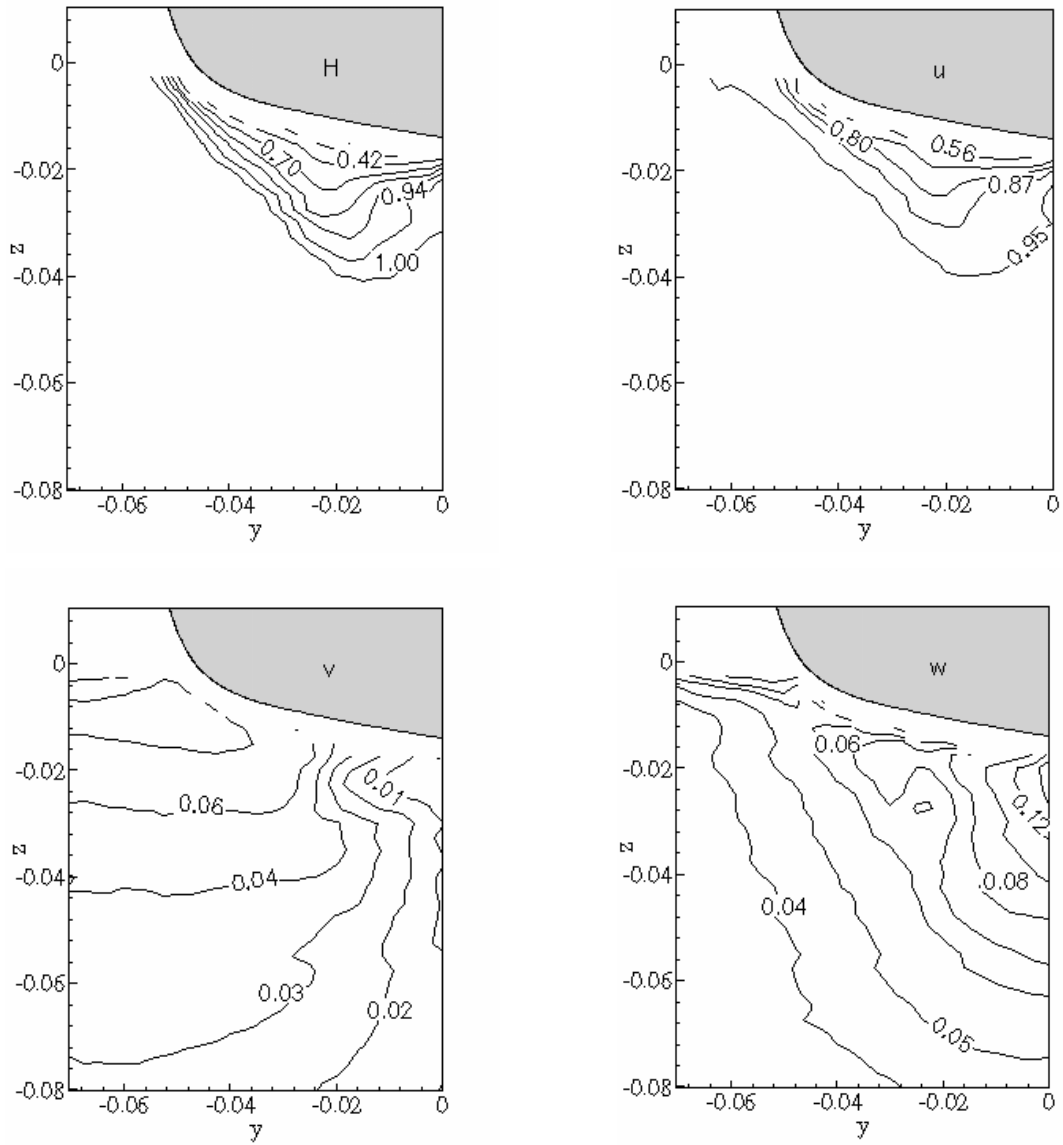
Fig. 28: propeller plane results as iso-levels of total head (H) and velocity components.
