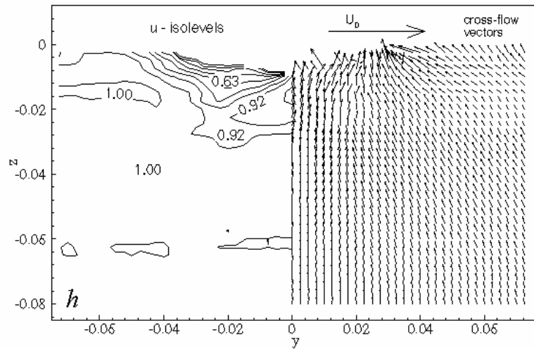
Fig. 18h: longitudinal velocity component iso-levels ( left ) and cross-flow vectors ( right ). Cross-section x = 1.0 : (port side measurements and mirror).
