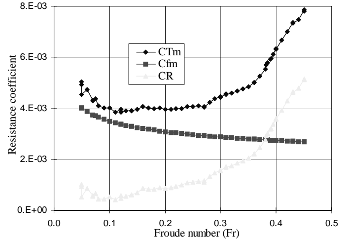
Fig. 3: Total, viscous and residual resistance coefficients as a function of Froude number
