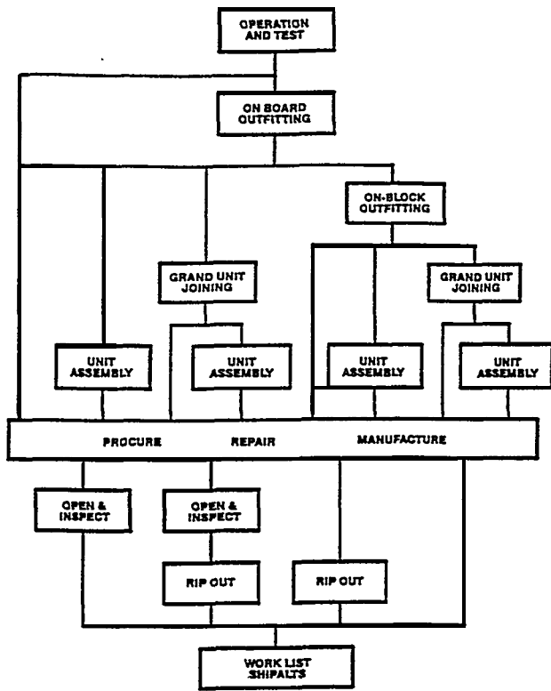
FIGURE 9a: Typical work flows by problem area for ship modernization.
