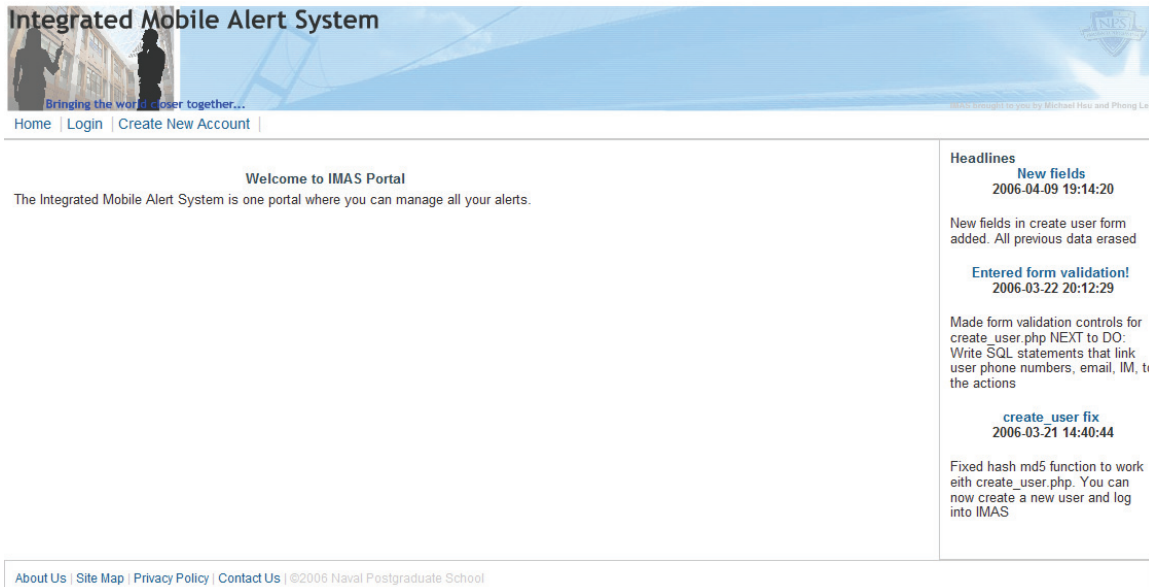
Figure 11. IMAS Homepage
