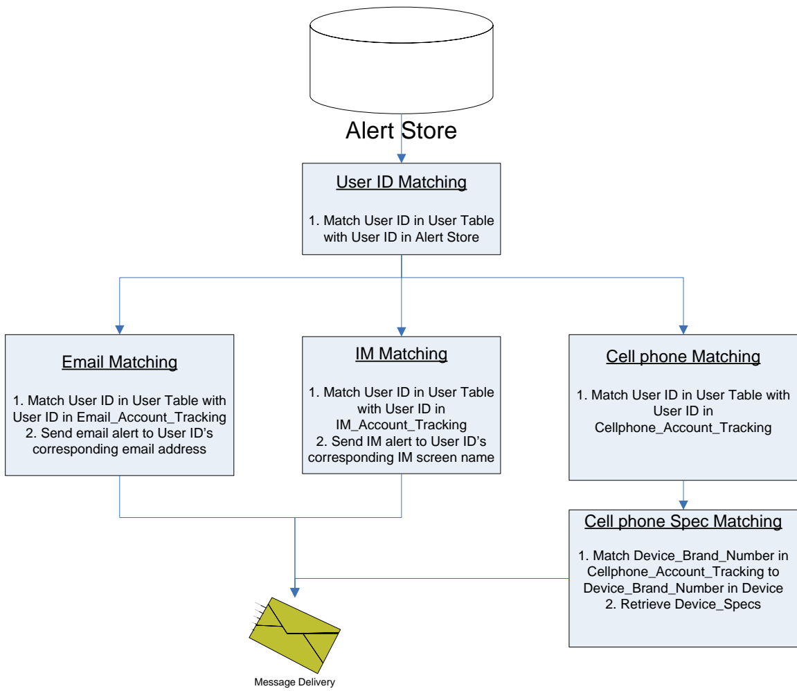
Figure 6. Message Delivery
