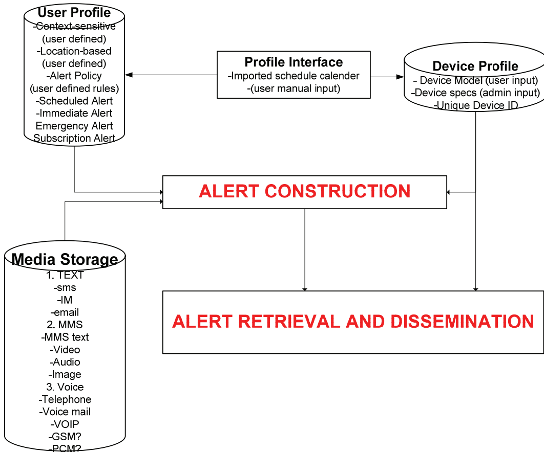
Figure 1. IMAS Framework
