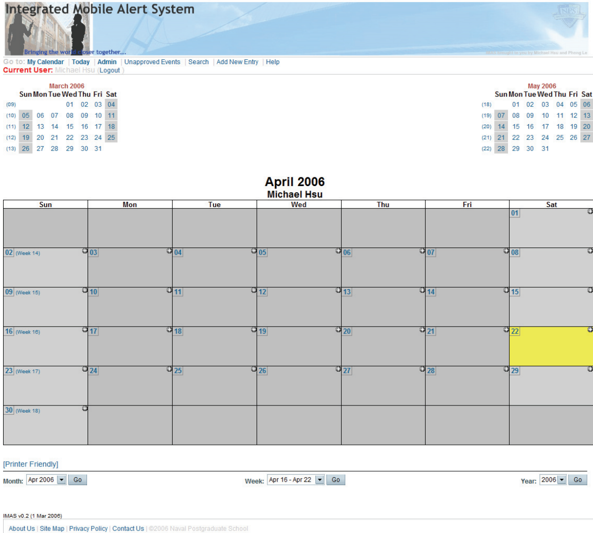
Figure 3. Calendar View
