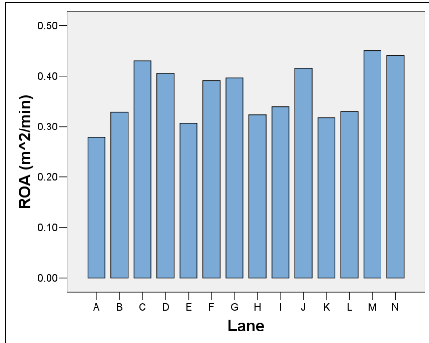
Figure E-1. Median Rate of Advance versus Lane for all Trials.
