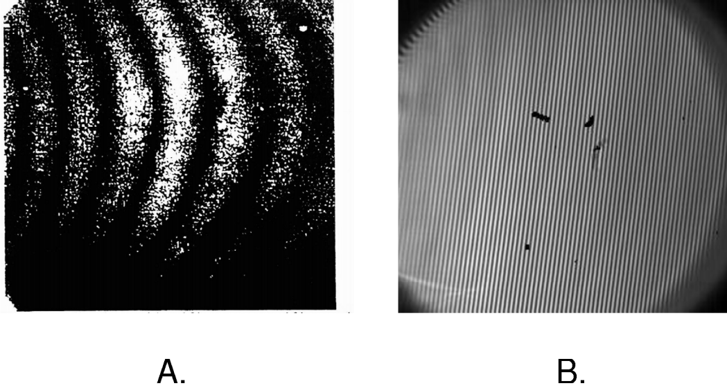
Figure 12: LWIR fringes recorded at LANL in panel A [Laubscher et al., 1999] compared to a typical fringe pattern recorded at NRL with the SHIMCAD breadboard interferometer in panel B. The NRL data was cropped to 256 horizontal pixels to match the LANL detector. The defects in panel B are due to bad pixels in the detector array.
