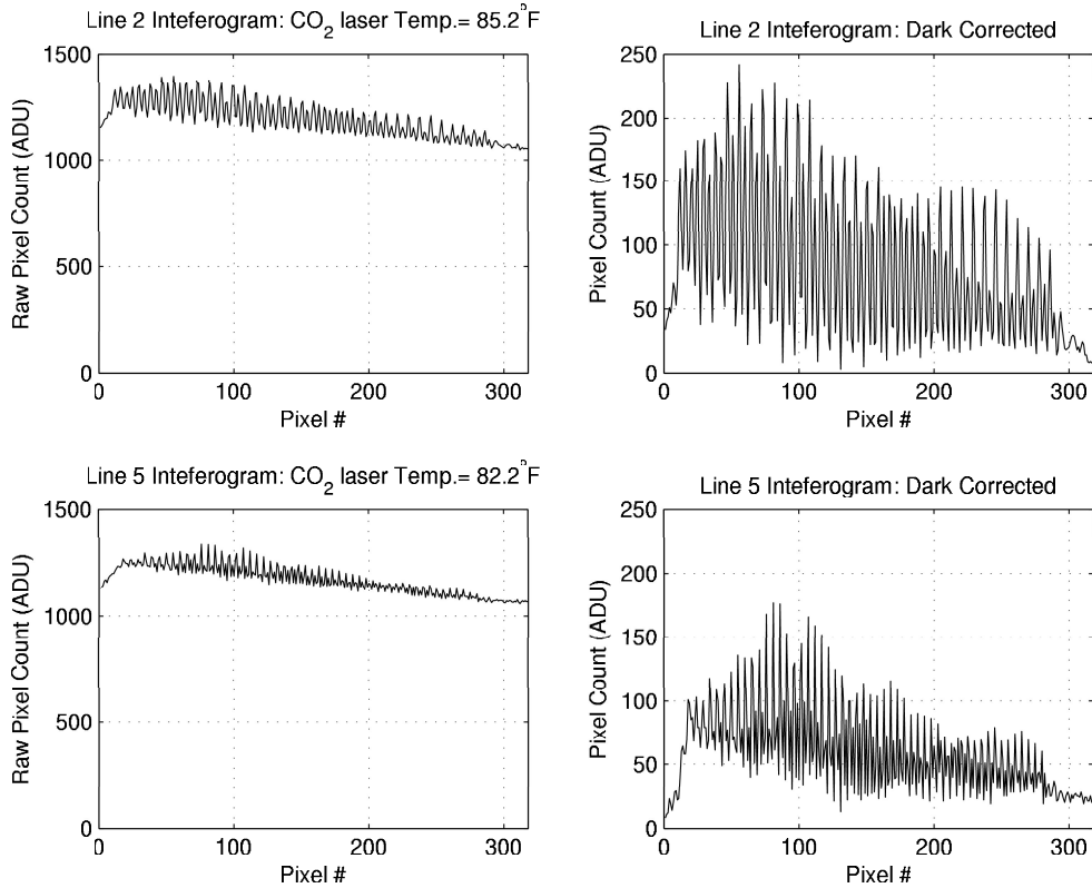
Figure 9: The two left panels show raw interferograms for two CO 2 laser lines (top: \lambda = 10.653 \mu\text{m} , bottom: \lambda = 10.303 \mu\text{m} ). Each interferogram represents a vertical row (slice) of the 2D microbolometer array. The laser tuning was achieved by changing the cavity temperature. The two right panels show the same interferograms after subtracting the background signal that does not originate from the laser (laser on minus laser off). Most of the subtracted nonmodulated signal is due to the fact that the detector field of view is not matched to the interferometer output beam for this breadboard set-up.
