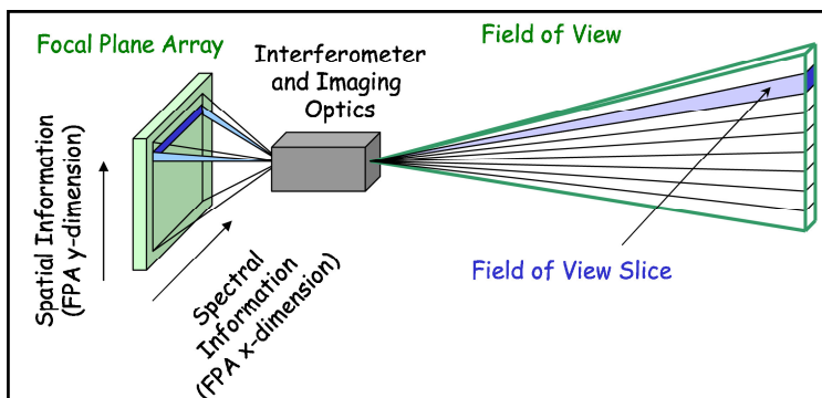
Figure 2: Viewing geometry concept: The field of view (FOV) is composed of slices. The signal of each slice forms a complete interferogram in the x-dimension of the focal plane array. In order to guarantee that the spatial structure of the scene within a FOV slice does not contaminate the interferogram, an anamorphic telescope is used, which causes the scene to be out of focus in the x-dimension but in focus in the y-dimension of the FPA.
