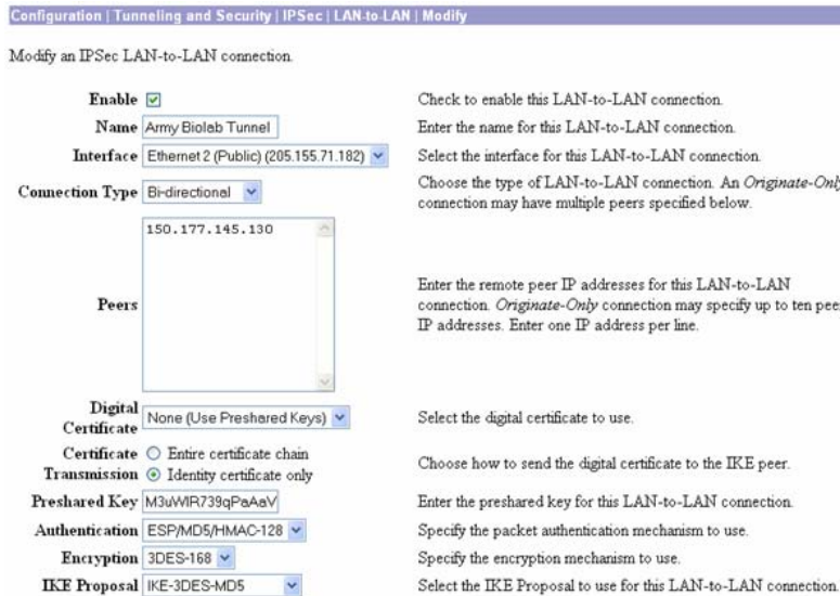
Figure 16. IPsec L2L Config TNT 06-2 (BFC)
