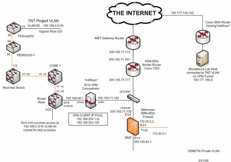
Figure 6. TNT Architecture prior to TNT 06-2.
