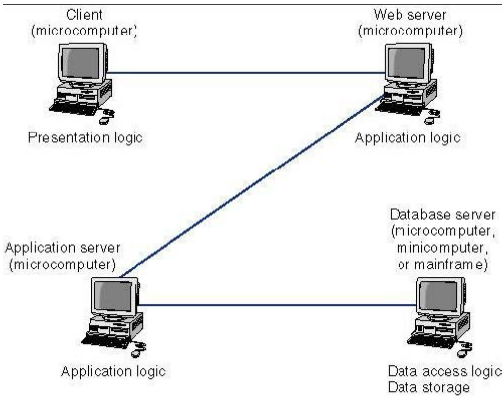
Figure 3. Four -Tier Architecture Diagram. [From Ref 18]
