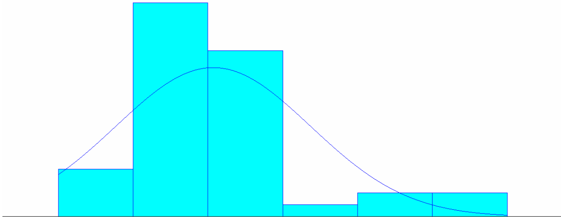
Figure 3. Total demands distribution with normal expression: NORM[825,508] (From [16])
