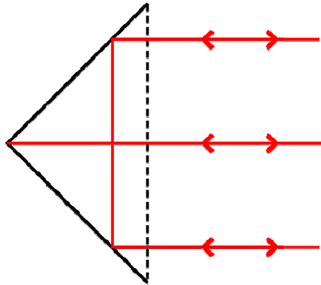
Aperture of Trihedral
