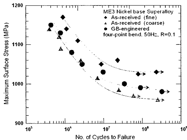
Fig. 11: Stress/life (S/N) curves (in 25°C room air at R = 0.1 , 50 Hz) for the nickel-base superalloy ME3 in three microstructural conditions: as-received (fine grained: D_g \sim 1.3 \mu\text{m} , coarse grained: D_g \sim 15 \mu\text{m} ) and GB-engineered ( D_g \sim 13 \mu\text{m} ).
