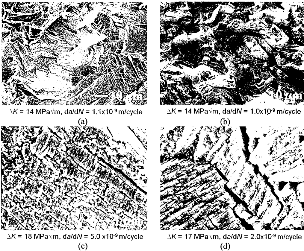
Fig. 5: SEM fractography of ambient temperature fatigue-crack propagation in ME3 at near-threshold stress intensities, for (a,c) as-received and (b,d) grain-boundary engineered microstructures.
