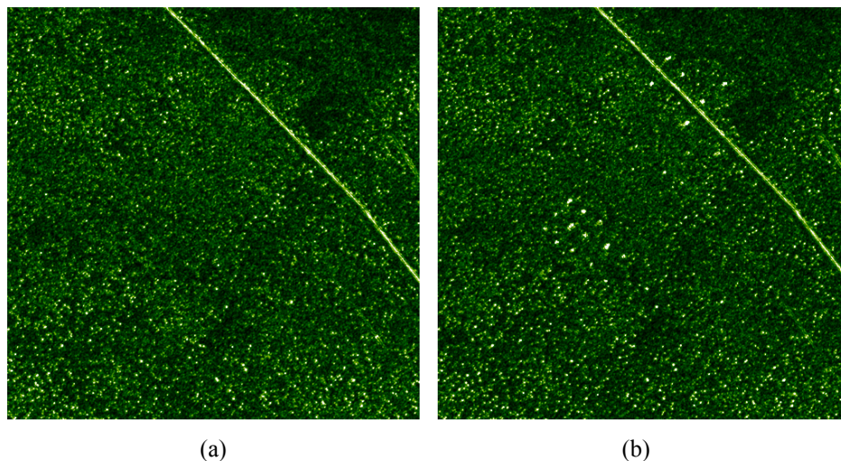
Figure 6: Example of a CARABAS-II SAR change detection image pair: (a) Reference image from 3 June with no targets; (b) Surveillance image from 7 June with 25 concealed targets.
