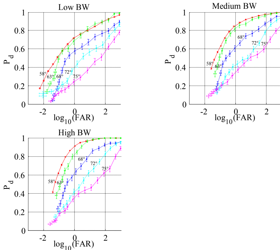
Figure 10: ROC curves for study two showing performance as a function of incidence angle for various bandwidths. The 58°, 63°, 68°, 72° and 75° incidence angle results were generated using 68, 4, 4, 4, and 4 image pairs, respectively. There were only 200 targets available for the 75°, 72°, 68° and 63° cases whereas the 58° case had 3400 target available. FAR is given in \text{km}^{-2} .
