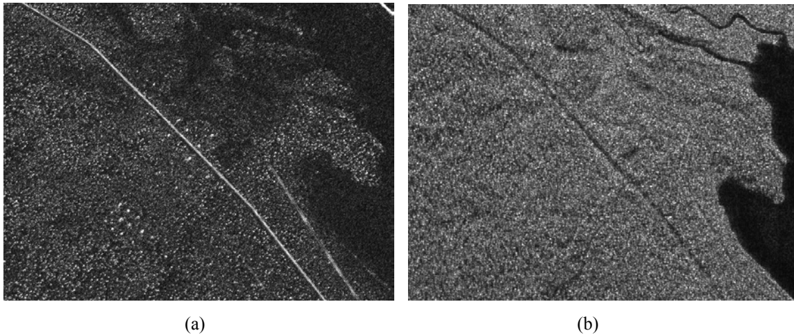
Figure 5: SAR images of targets deployed in a forest during Vidsel'02. (a) CARABAS-II (20-86 MHz) SAR image with 2.5-m resolution. The bright linear feature running diagonally across the image is a power line along the road. Note the targets visible along the road and deeper inside the forest. (b) K_u -band SAR image covering the same area with 3-m resolution. Targets in the forest were deployed but are not visible in the image.
