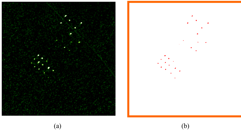
Figure 7: CARABAS-II SAR change detection result from the image pair in Figure 6. (a) Change image based on linear Bayesian classification; (b) After CFAR detection.
