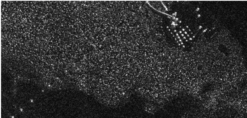
Figure 3: CARABAS-II (20-86 MHz) SAR image (2.5-m resolution). 25 vehicles of different sizes and orientations as well as a few buildings are clearly visible in the open field.
