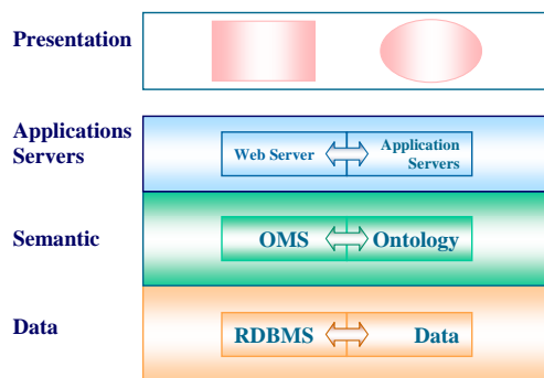
Figure 1. N-Tier Architecture
