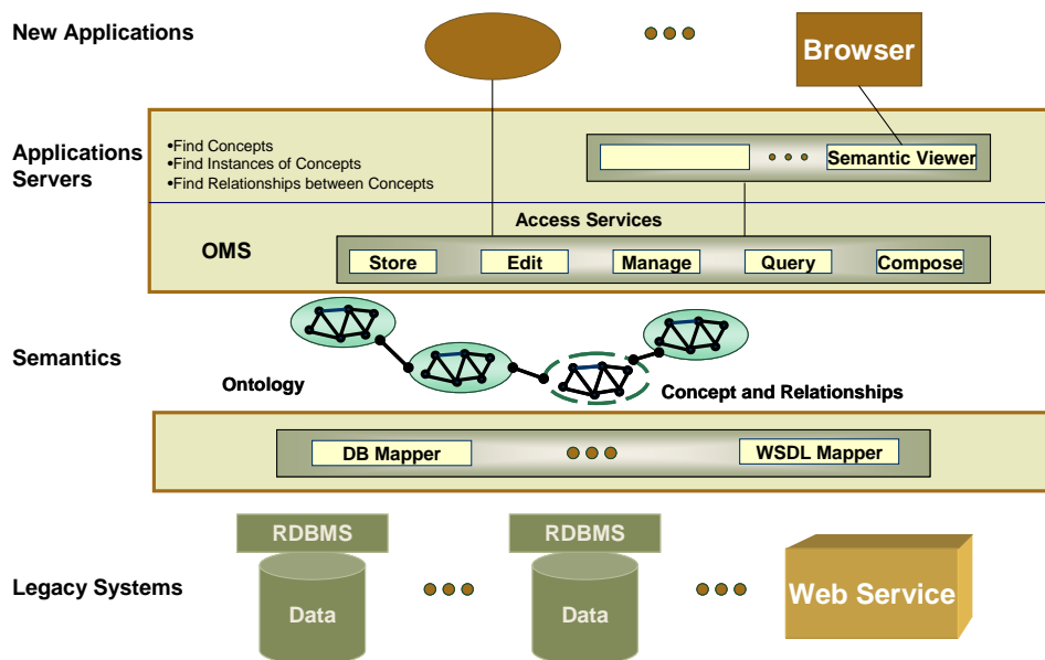
Figure 12. Ontology-Based Architecture
