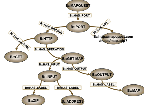
Figure 9 - Mapquest Meta-Ontology
