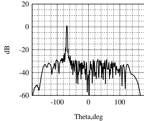
Figure 6. 97-Element Large Semicircular (ls) Array Pattern, GA Method, P3N Mask, Taper Effic = -4.4 dB We = 0.5
