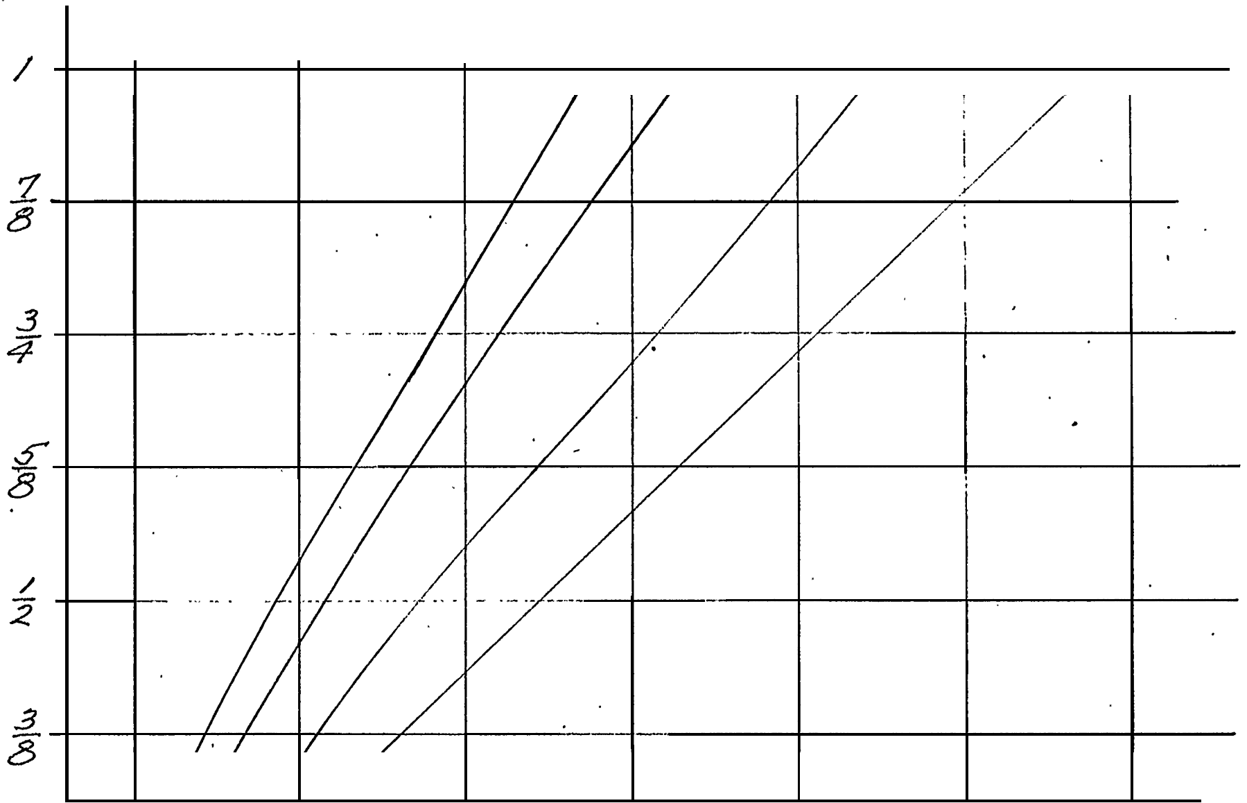
APPROX. DOLLAR SAVINGS FOR EACH % INCREASE - PART YIELD FROM CARBON STEEL PLATE (MAT'L ONLY)
