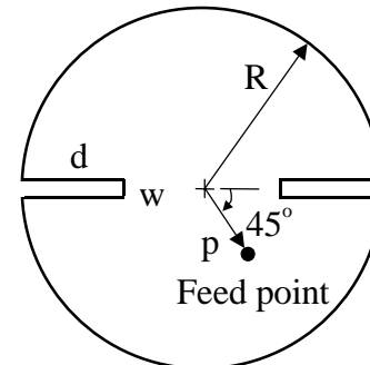
Figure 2. Single-Slot Patch
