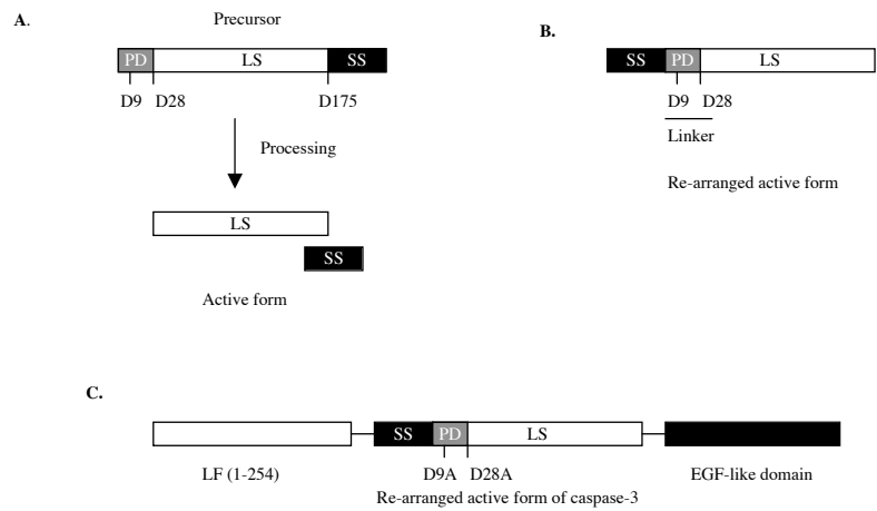
Fig. 4. Use of re-arranged active form of caspases in a cellular delivery system. A. Shown is the processing of caspase-3, where the two subunits (LS and SS) in the active form of the enzyme are marked. Also marked are the aspartate (D) processing sites; PD, prodomain. B. Re-arranged, constitutively active form of caspase-3 that does not require processing. C. Hybrid protein for cellular delivery tests. The aspartate processing sites in the linker region of the re-arranged caspase-3 will be mutated. The hybrid protein also contains the domain of anthrax LF (residues 1-254) that is sufficient for cellular translocation [1] and the EGF-like domain for cancer cell targeting. Not shown are protein tags that can facilitate protein purification. Diagrams not drawn to scale.
