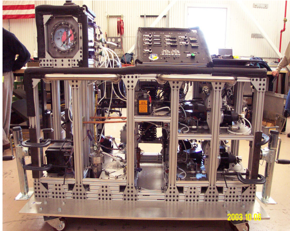
Fig. 2 Experimental apparatus.
