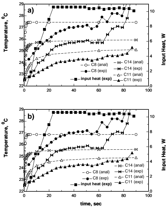
Fig. 16 Comparison of analytical calculation results to experimental results a) h_1=18,000 , h_3=250 , f=0.01 b) h_1=22,000 , h_3=250 , f=0.01 .
