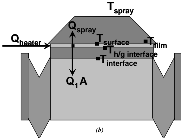
Fig. 10 Heater and heater support structure region a) radial and axial thermocouple locations b) schematic of heat and fluid flow paths with critical temperature locations.
