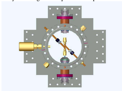
Fig. 3 Spray test chamber.
