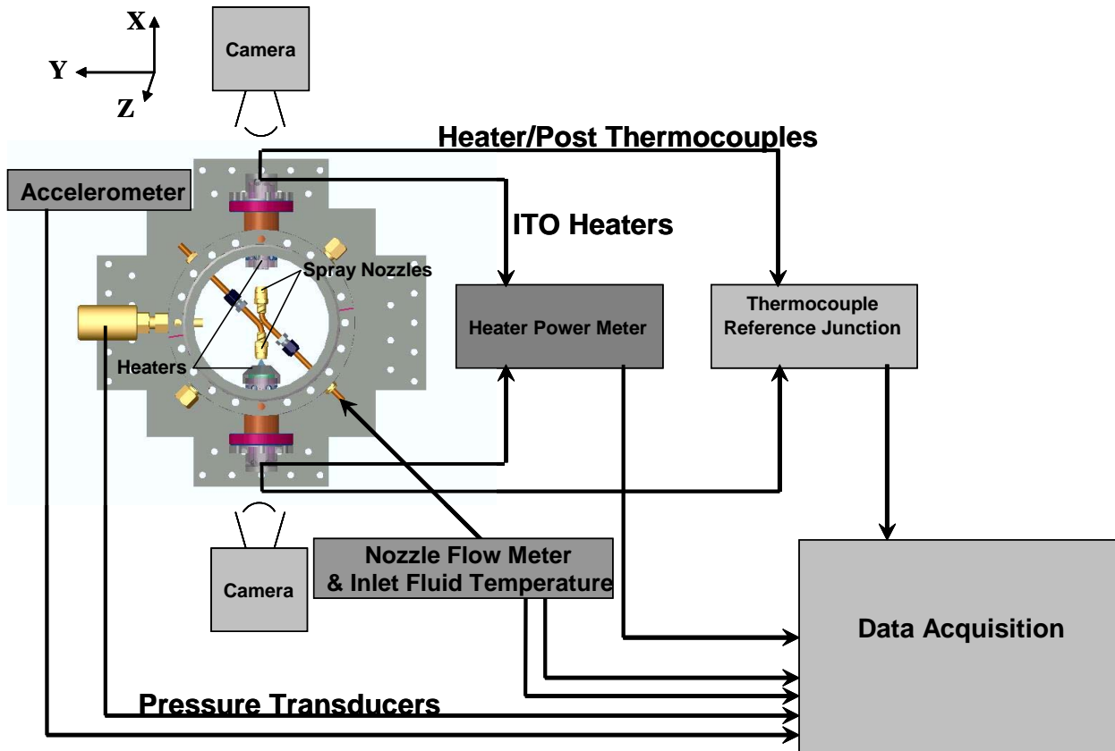
Fig. 9 Instrumentation schematic.
