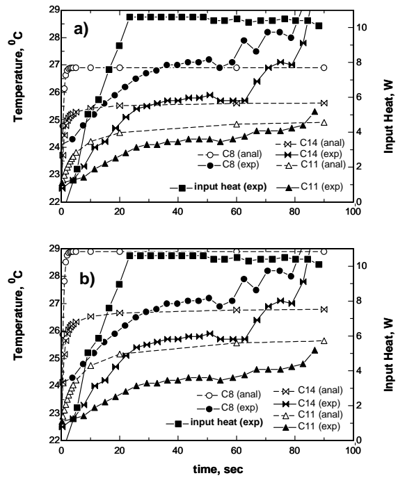
Fig. 18 Comparison of analytical calculation results to experimental results a) h_1=20,000 , h_3=250 , f=0.005 b) h_1=20,000 , h_3=250 , f=0.05 .
