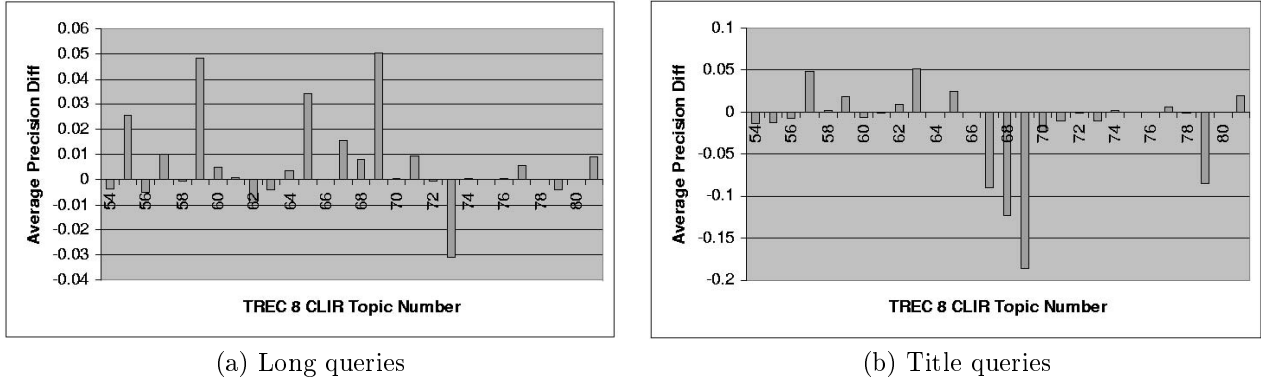
Figure 1: Comparative results by query, merged monolingual. (a) Pirkola’s method better above zero, DQT-ET better below. (b) Pirkola’s method better above zero, DQT-ET better below.
