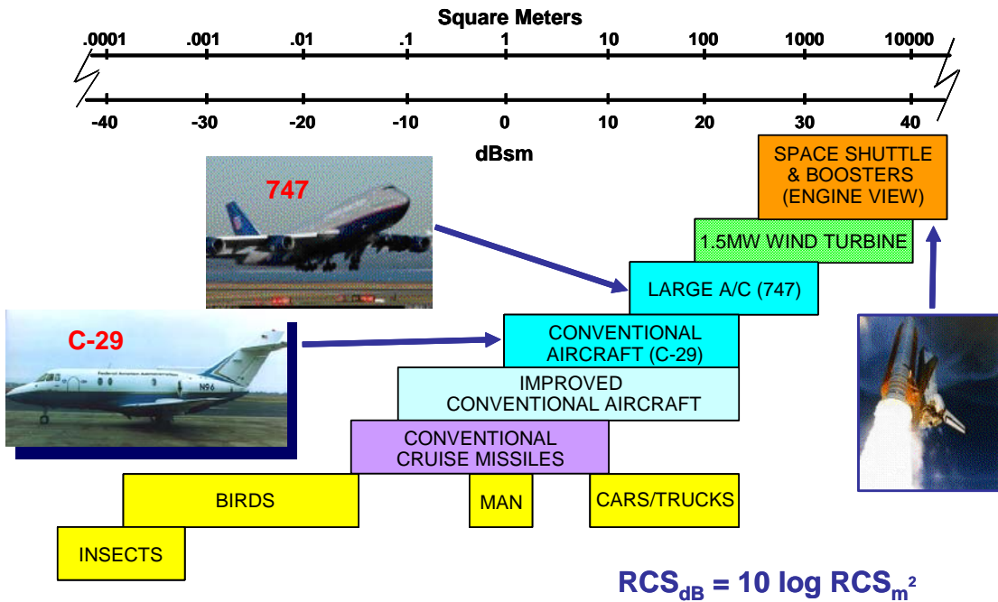
Figure 7. RCS values for several common objects
