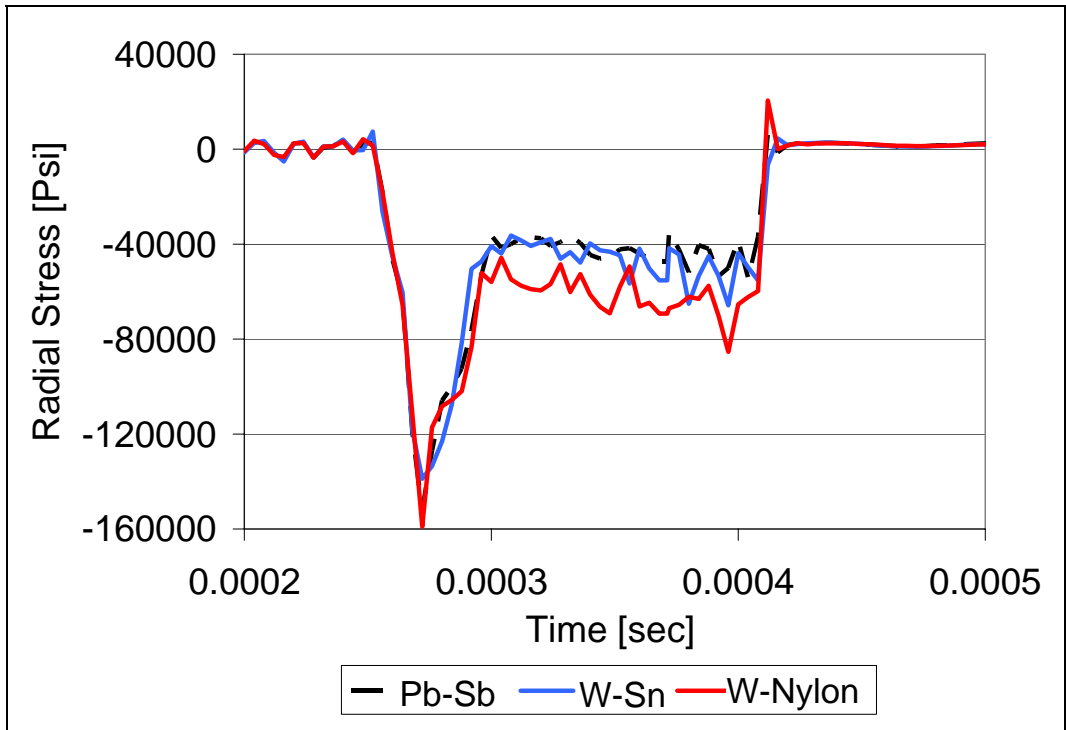
Figure 8. Predictions of the radial stress on the land at the origin of rifling for each slug material.
