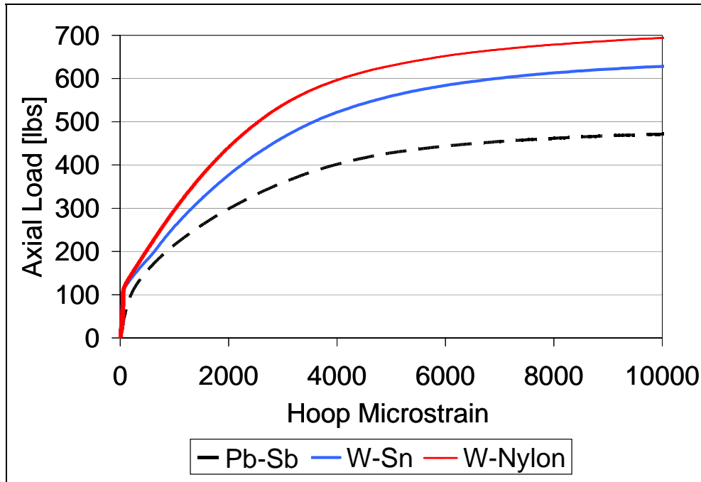
Figure 5. Plot of the average response of the sheathed slug test for each of the three materials.
