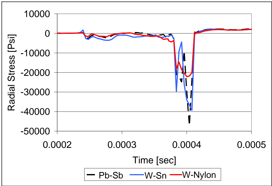
Figure 9. Predictions of the radial stress on the groove at the origin of rifling for each slug material.
