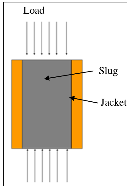
Figure 3. Schematic of the testing arrangement showing the sheathed slug. The arrows denoted the loading direction.
