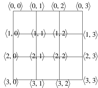
Figure 1: Single grid protocol: A node marked \langle j, k \rangle is associated with user u_{\langle j, k \rangle} and grid secret k_{\langle j, k \rangle}
