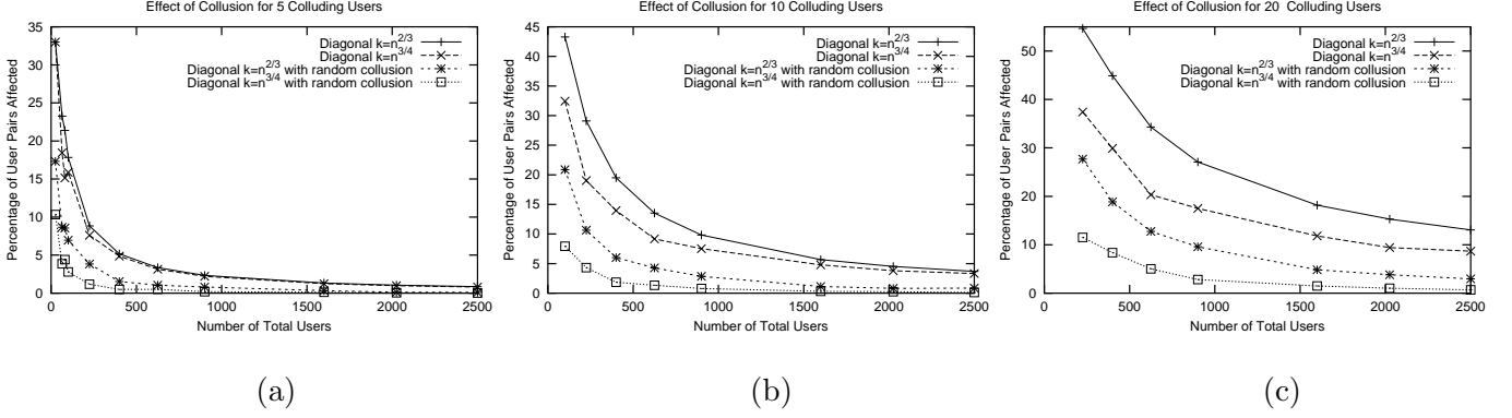
Figure 5: Collusion in diagonal protocol for different k values. (a) 5 colluding users (b) 10 colluding users and (c) 20 colluding users
