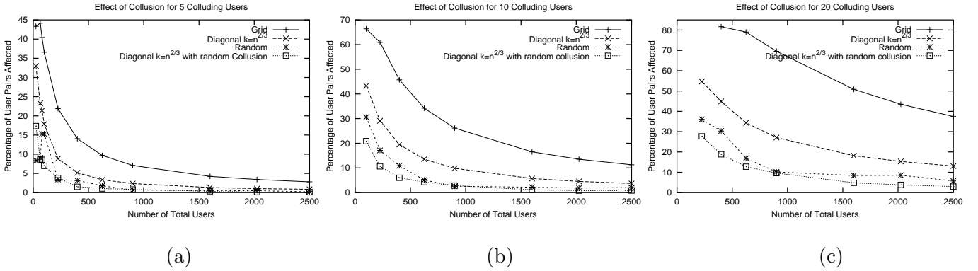
Figure 4: Effect of collusion on various protocols. (a) 5 colluding users (b) 10 colluding users and (c) 20 colluding users
