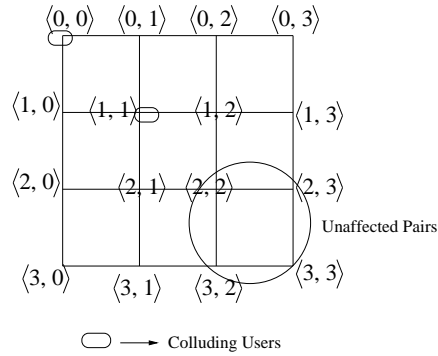
Figure 2: Effect of Collusion on Grid Protocol
