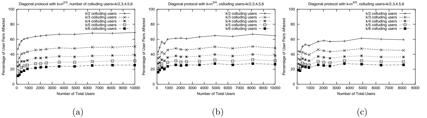
Figure 6: Collusion in diagonal protocol for k/X colluding users. (a) k = n^{2/3} (b) k = n^{3/4} (c) k = n^{4/5}
