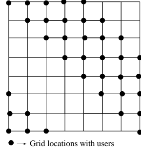
Figure 3: User assignment in the diagonal protocol
