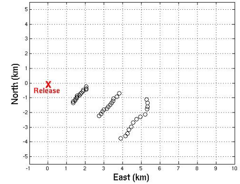
4/30/79 Active Sampler Locations
