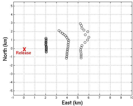
6/27/79 Active Sampler Locations
