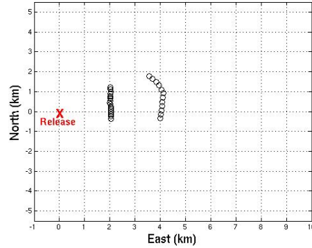
11/9/78 Active Sampler Locations
