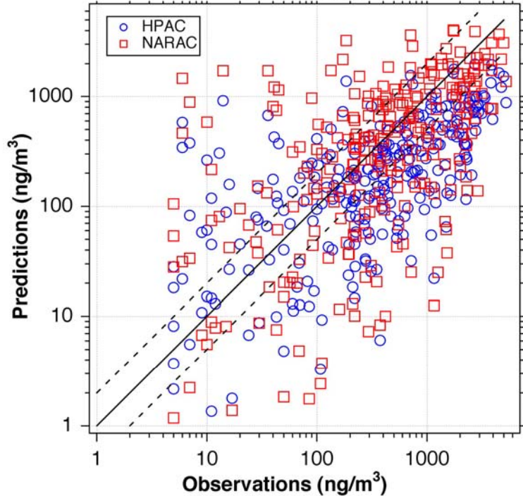
1 Hour Average Predictions vs Observations: All Releases
