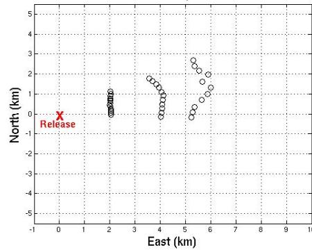
7/6/79 Active Sampler Locations
