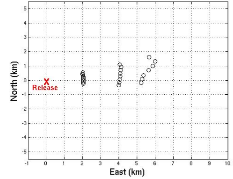
7/19/79 Active Sampler Locations
