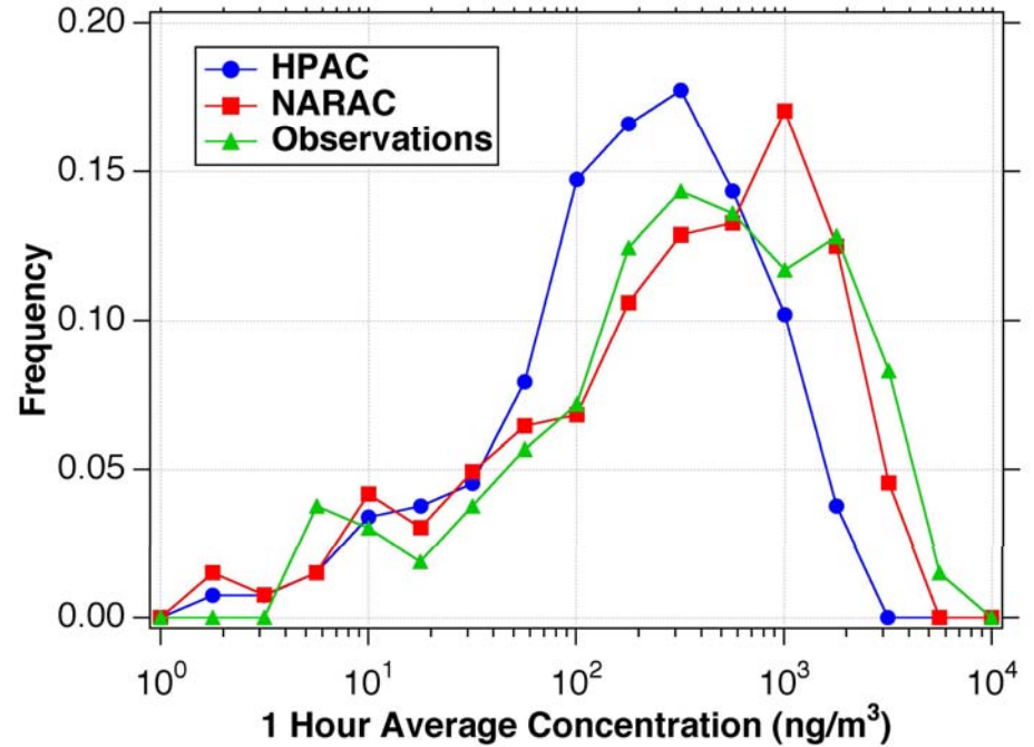
Histogram Comparison: 1 Hour Average Concentrations
