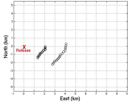
11/3/78 Active Sampler Locations
