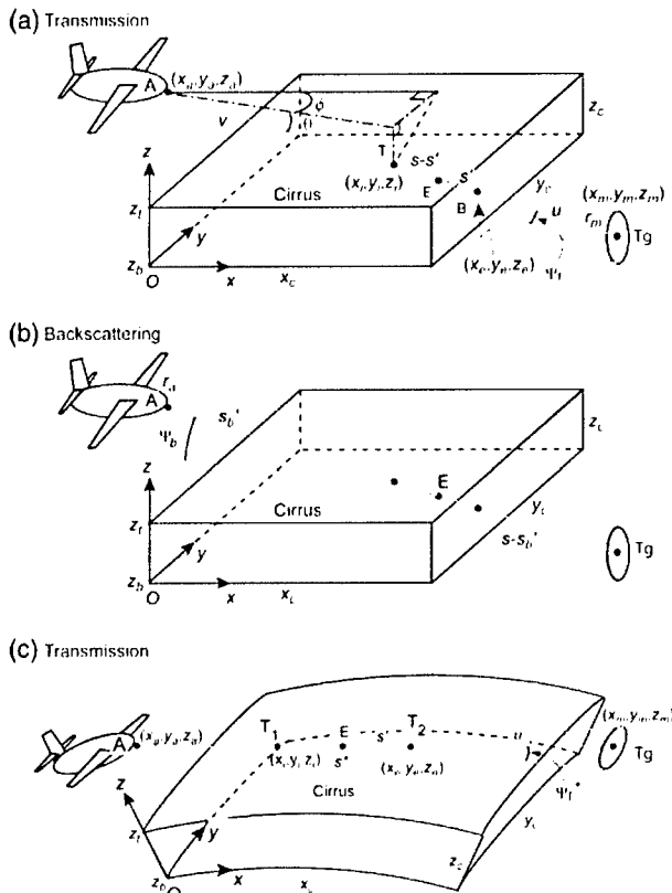
Fig. 3. (Color online) (a) Laser transmission through a 3D cloud. The positions $(x_a, y_a, z_a)$, $(x_m, y_m, z_m)$, $(x_i, y_i, z_i)$, and $(x_e, y_e, z_e)$ denote coordinates of the airborne laser, target, incident point, and exit point; $(x_c, y_c, z_c)$ is the 3D cloud dimension, where $z_c = z_t - z_b$; $\theta$ is a laser scan angle; $\phi$ is a horizontal azimuthal angle; $\psi_1$ is an angle subtended by the target at point $E$; $r_m$ is the effective radius of the target; $s' = EB$; $u = BTg$; $v = AT$; and $s - s' = ET$. (b) Laser backscattering through a 3D cloud. $\psi_b$ is the angle subtended by the aircraft at point $E$, $r_a$ is the effective radius of the aircraft, $s - s_b' = ETg$, and $s_b' = EA$. (c) Laser transmission through a 3D inhomogeneous cloud in a spherical atmosphere. All symbols are the same as in (a), except that $s^* = T_1T_2$, $s' = ET_2$, $u = T_2Tg$, and $\psi_1^*$ is an angle subtended by the target at point $E$.
