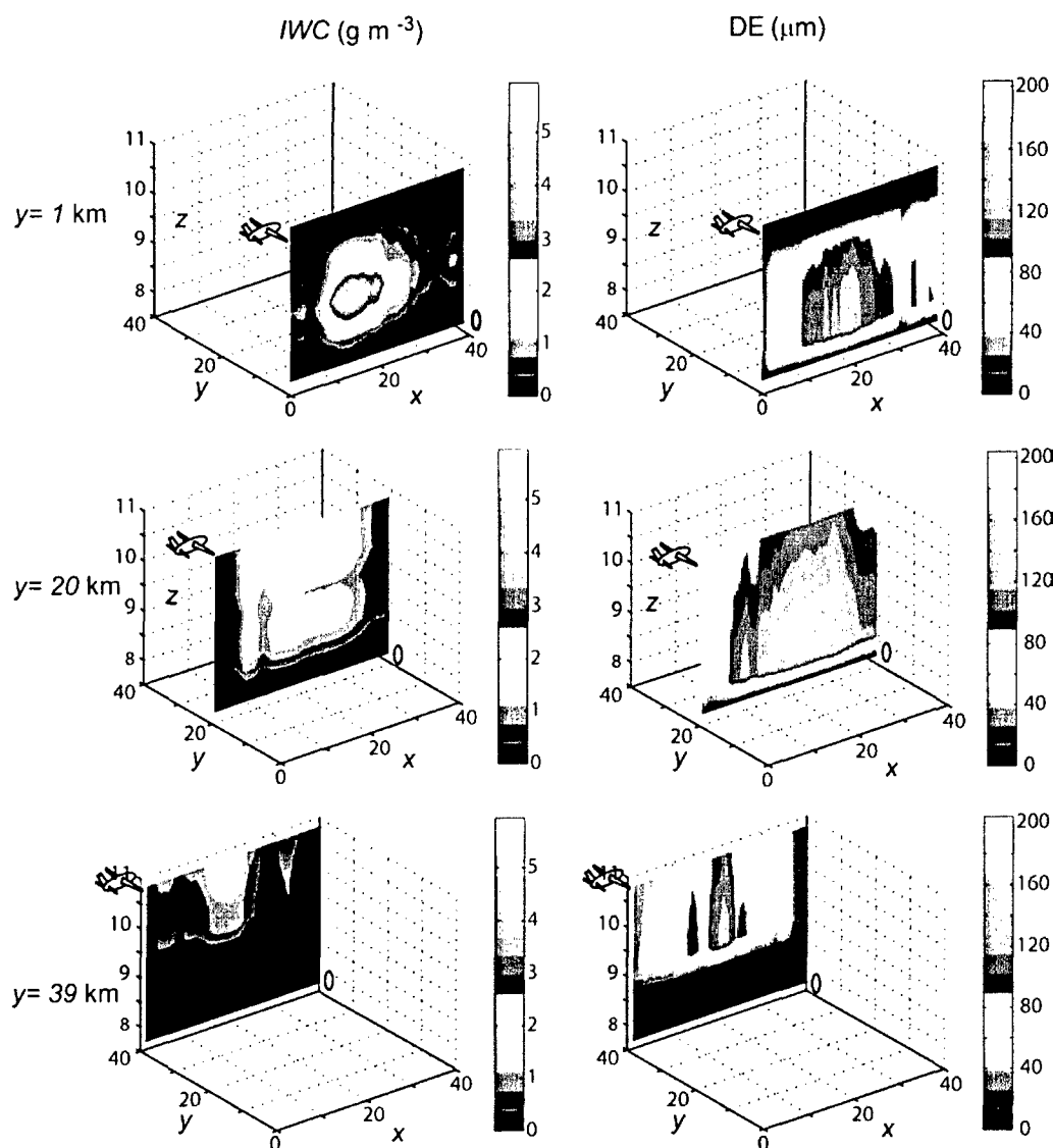
Fig. 4. (Color online) 3D cirrus IWC and DE fields mapped at y = 1, 20 , and 39 km obtained for the 18 April 1997 case over the ARM SGP Central Facility. The dark areas are areas with no observations. Also shown are the positions of the aircraft and the moving target.
