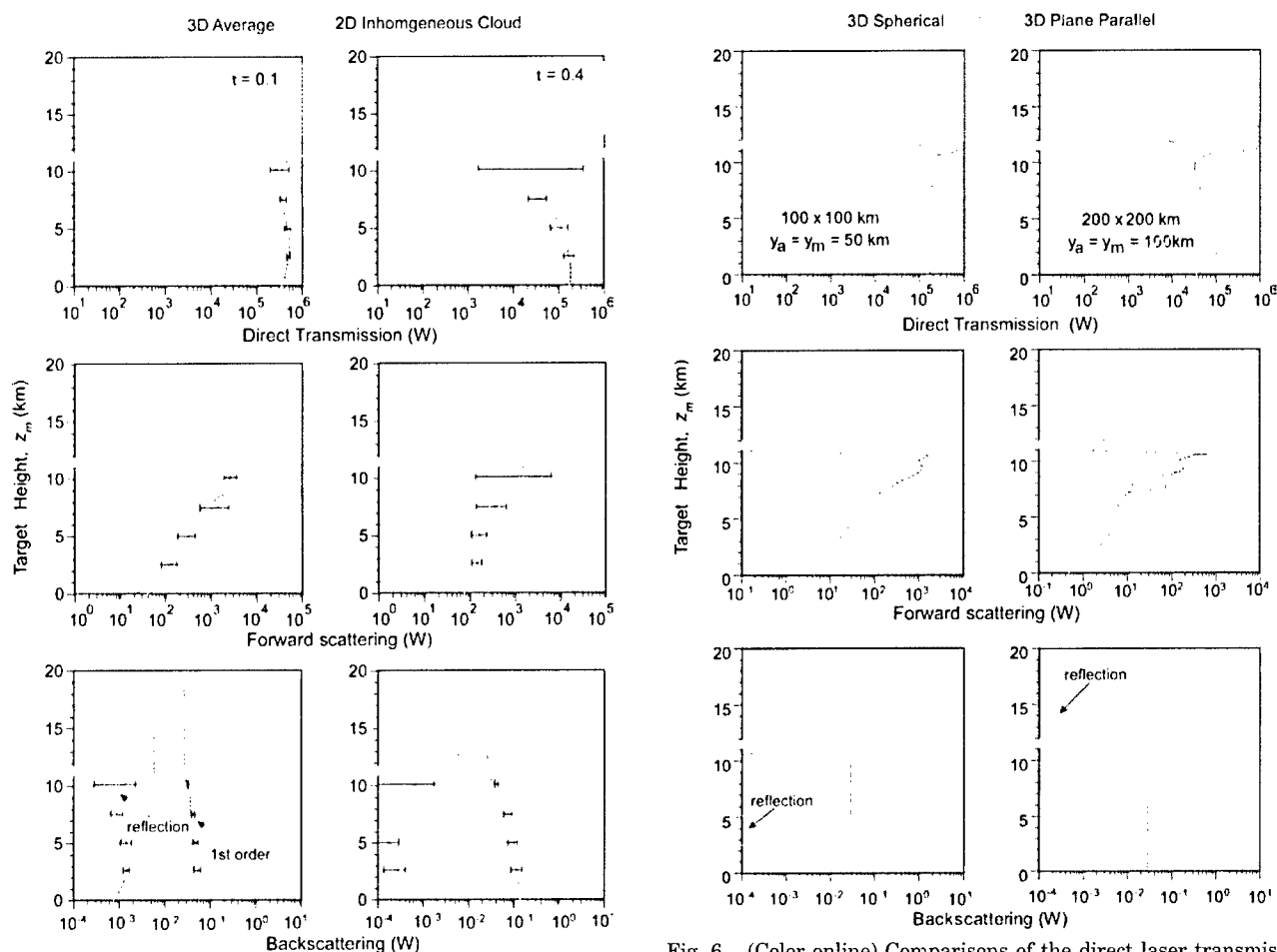
Fig. 5. (Color online) Direct transmission, forward scattering, and backscattering for a 2D inhomogeneous (averaged over the y direction) and mean values of those for the 3D cirrus cloud field based on the five vertical transects (1, 11, 20, 29, and 39 km) are displayed. Standard deviations of the 3D mean values based on the five 3D transect values are also plotted in terms of horizontal bars. \lambda = 1.315 \mu\text{m} , F_0 = 10^6 \text{ W} , R_\lambda = 0.2 , r_a = 4 \text{ m} , z_a = 11.2 \text{ km} , z_t = 11.1 \text{ km} , and z_b = 7.5 \text{ km} .
