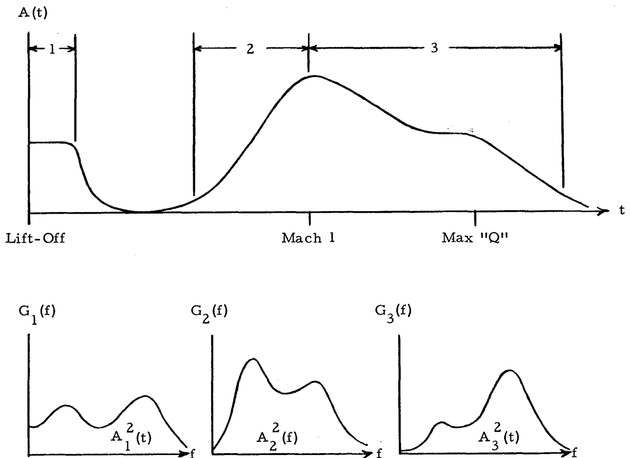
Figure 13. Spectral Representation for Spacecraft Launch Vibration Data
