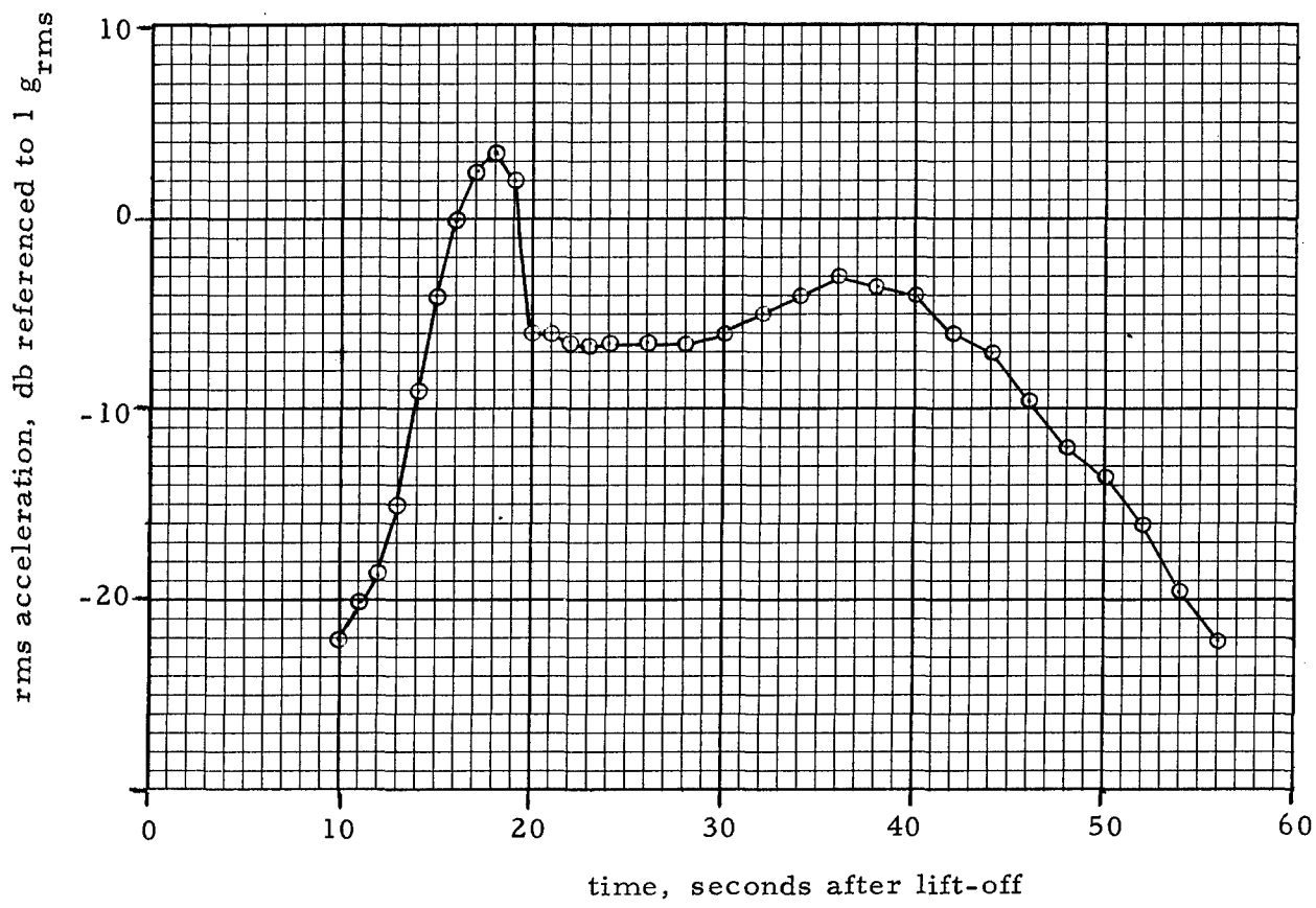
Figure C-17. Over-all rms Time History for MINUTEMAN Flight Vibration
