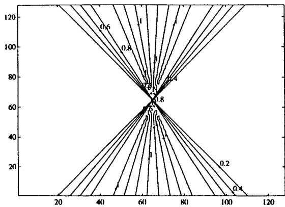
Figure 6: symbol q_0 .
