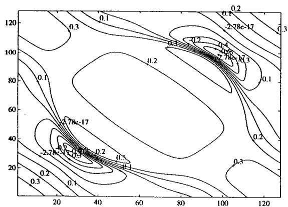
Figure 10: symbol rotation 2.
