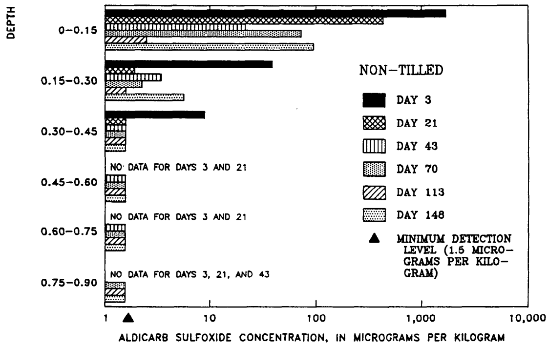
Figure 4. Median aldicarb sulfoxide for row-top position.
