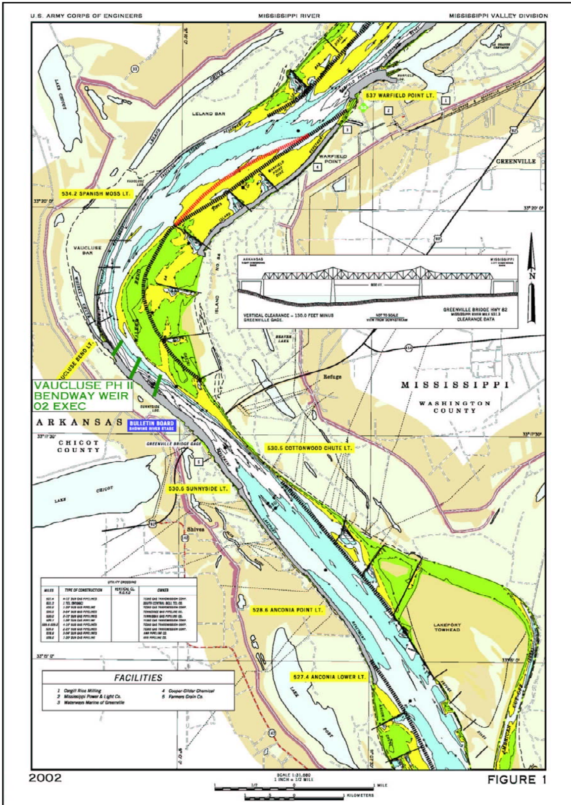
Figure 1. Vicinity map, Greenville Bridge Reach, bendway weirs, Mississippi River near Greenville, MS.
