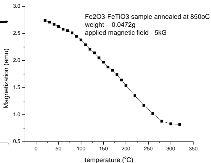
Fig.4. Magnetization of Fe-Ti ferrite as a function of temperature
