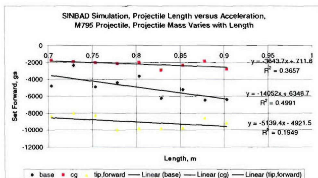
Figure 10 Results: SIMBAD analysis of the M795 projectile
