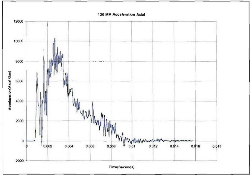
Figure 6 Acceleration time history of a typical projectile fired in a 120-mm mortar tube
