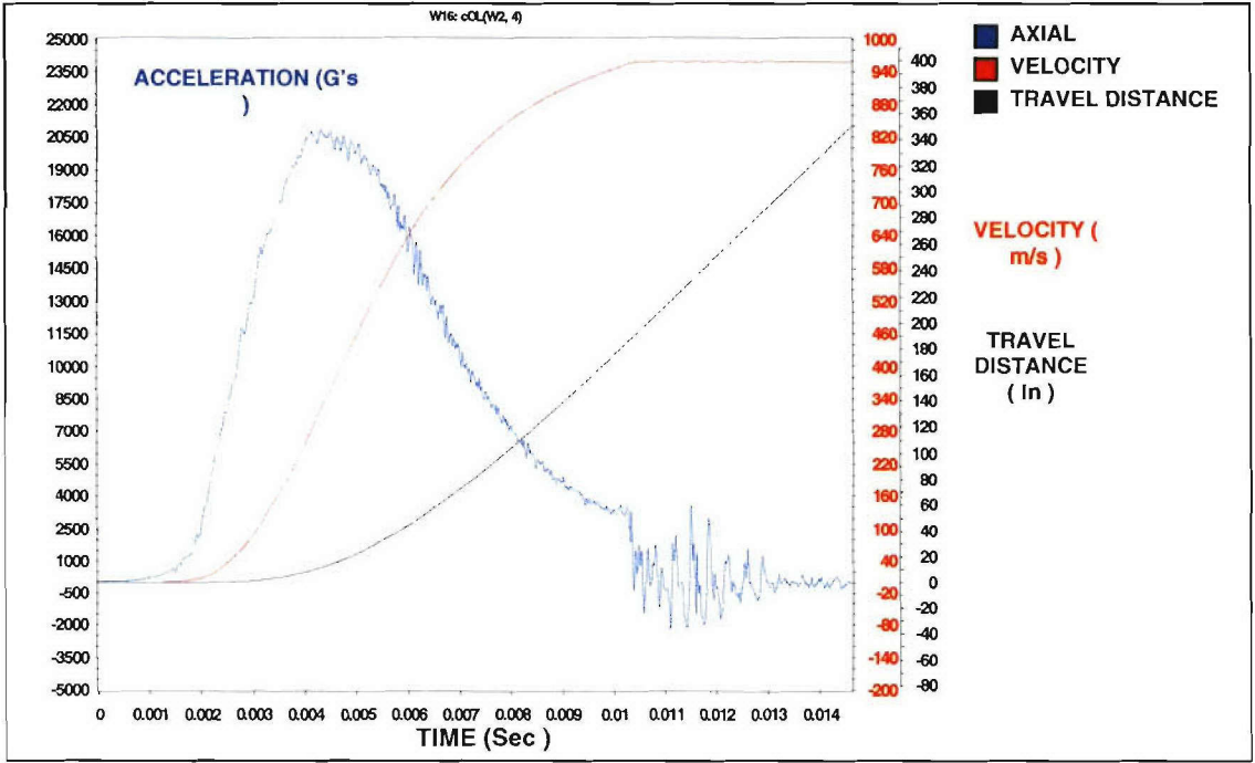
Figure 5 Acceleration time history of a typical projectile fired in a 120-mm tank cannon
