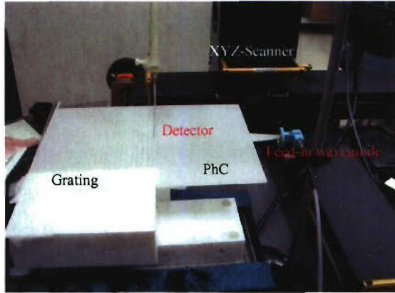
Fig. 10: Experimental setup for charactering the device.
