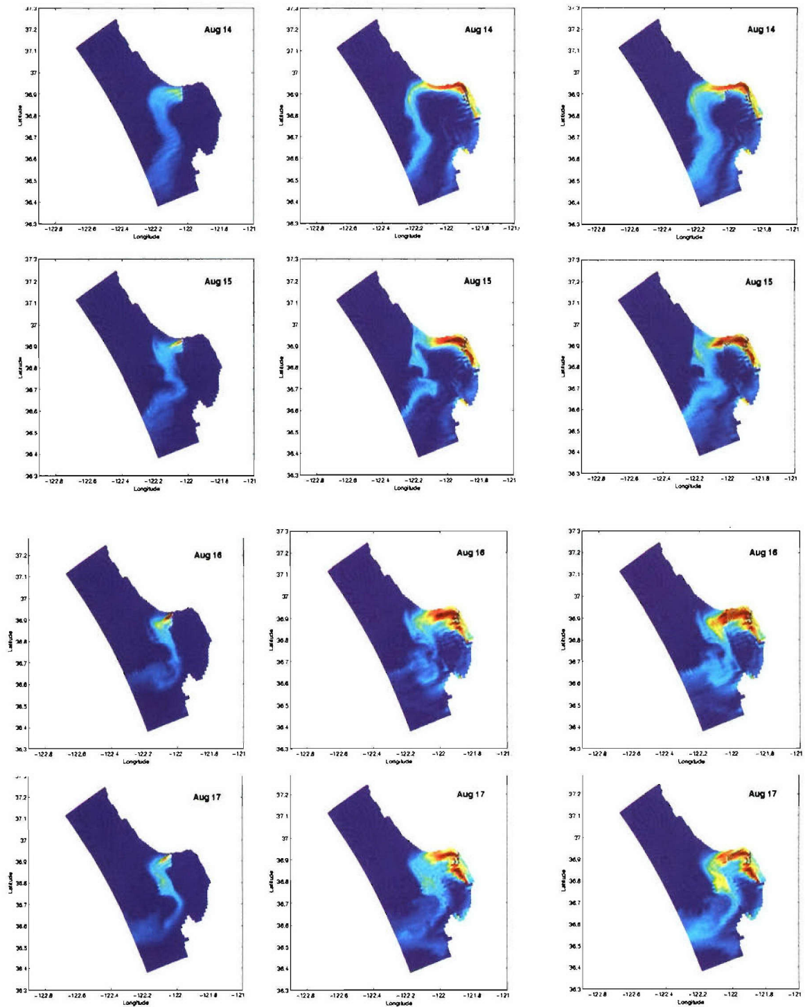
FIG. 9. Surface model-predicted bioluminescence distributions in three numerical experiments.
