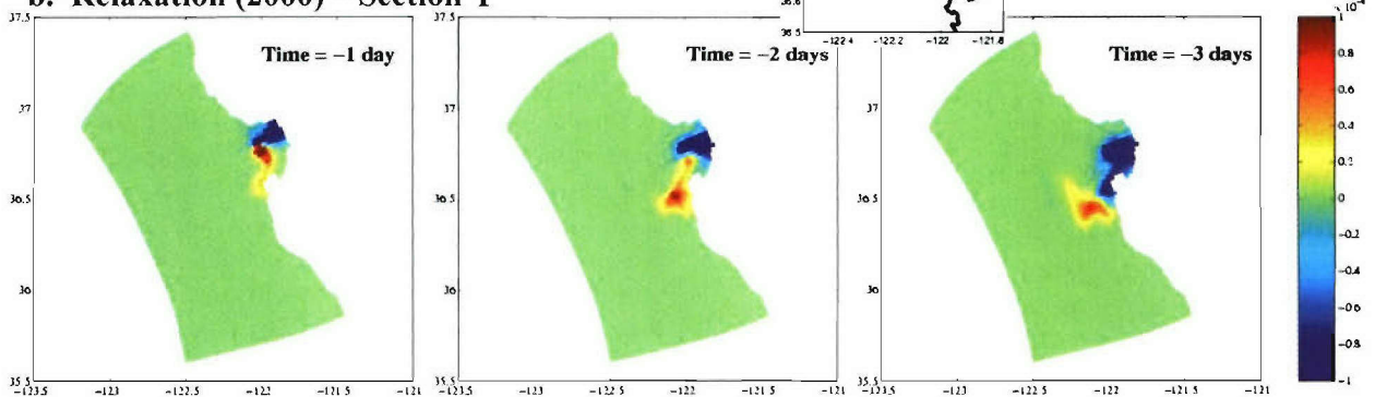
FIG. 6. Adjoint-based sensitivity maps for 1–3 days prior to the forecast during the relaxation event in Aug 2000 (a) at section X north of the bay; (b) at section Y in the northern part of the bay mouth.
