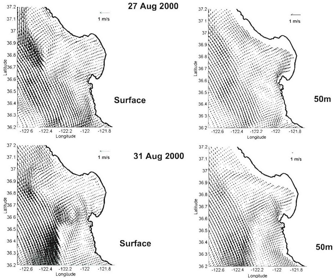
FIG. 2. ICON model surface and 50-m-depth currents during the wind relaxation event of 27–31 Aug 2000.
