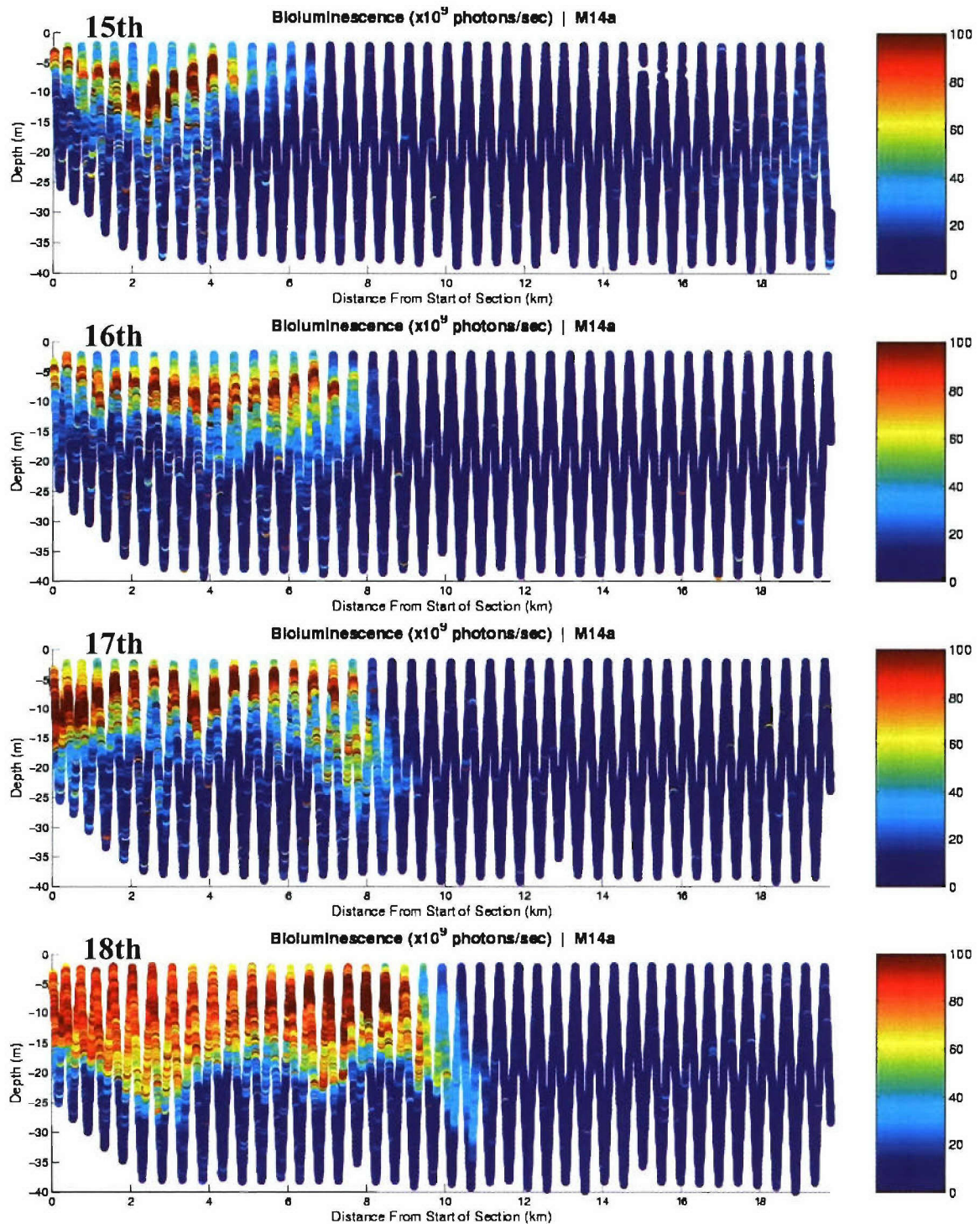
FIG. 5. Observed bioluminescence distributions along cross section M14a during 15–18 Aug 2003. The distance scale starts from the onshore end of the section.
