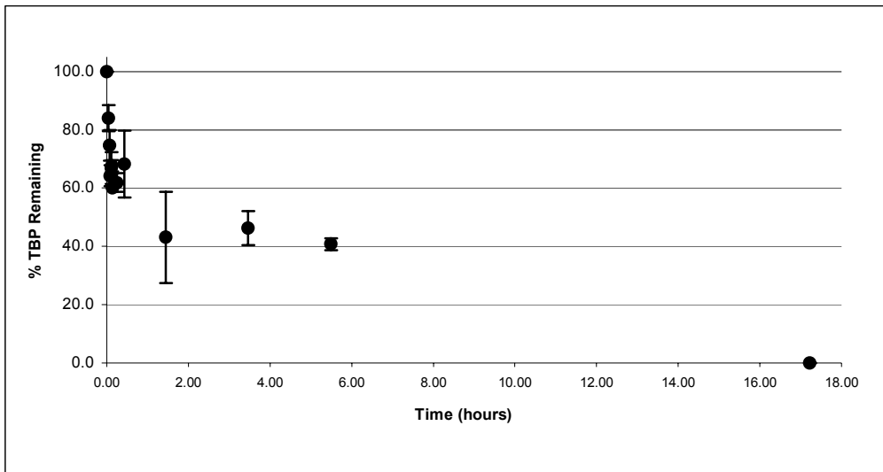
Figure 2: Decomposition of tributyl phosphate in acidic buffered alum solution.
