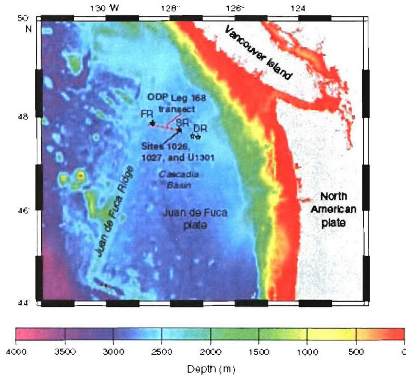
Figure F1 Regional bathymetric map showing major tectonic features and the locations of IODP Expedition 301 drill sites and the ODP Leg 168 drilling transect. Bathymetry from Smith and Sandwell (1997). FR = First Ridge, SR = Second Ridge, DR = Deep Ridge.
