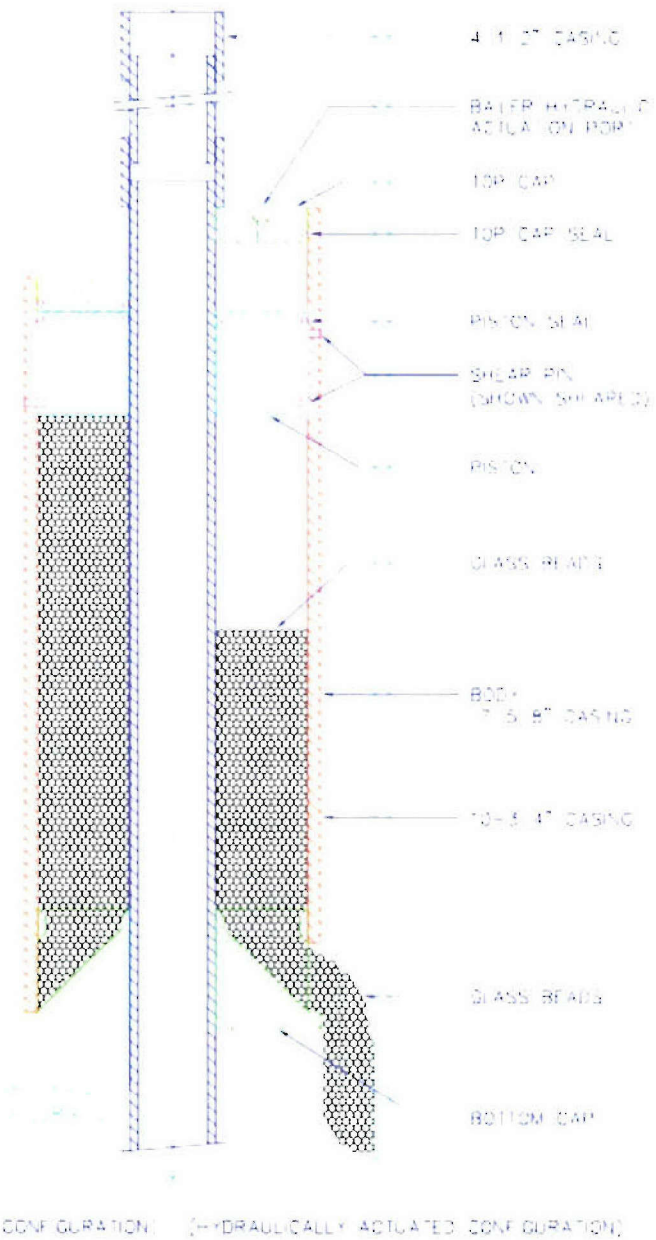
Figure 5. Hydraulically Actuated Bead Dump Bailer Concept.
