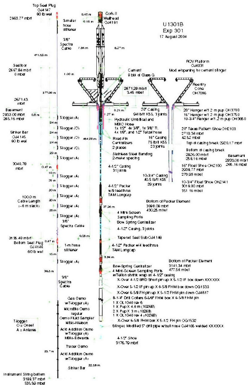
Figure F17. Schematic showing the Hole U1301B reentry cone and borehole casing (right), CORK borehole completion (center), and the instrument string deployed through the 4 1/2 inch casing (left). ROV = remotely operated vehicle.
