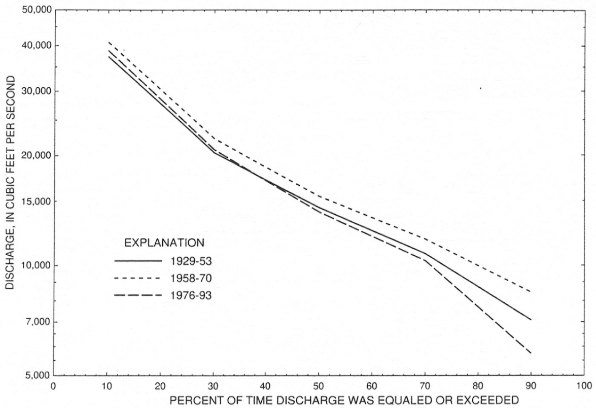
Figure 2. Flow-duration curves of inflow data for Lake Seminole near Chattahoochee, Florida.
