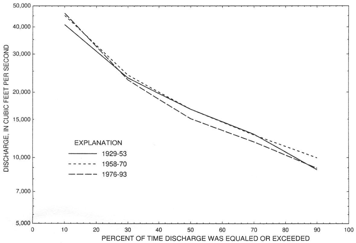
Figure 3. Flow-duration curves of outflow data for Lake Seminole near Chattahoochee, Florida.
