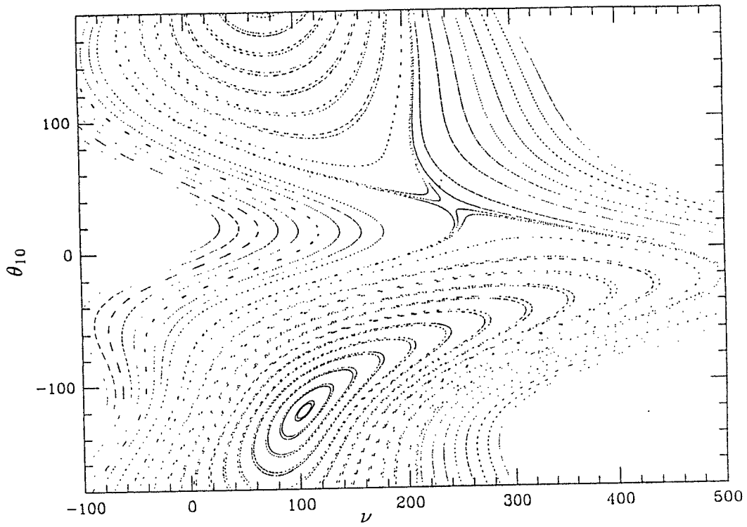
(a) \lambda = 0
