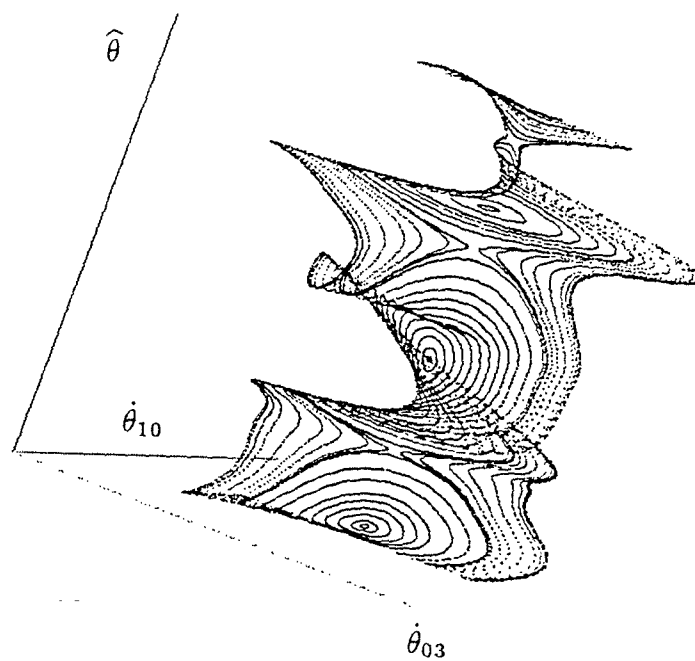
(b) \lambda = 0
