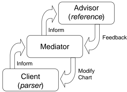
Figure 1: A General Architecture for Incremental Parsing
