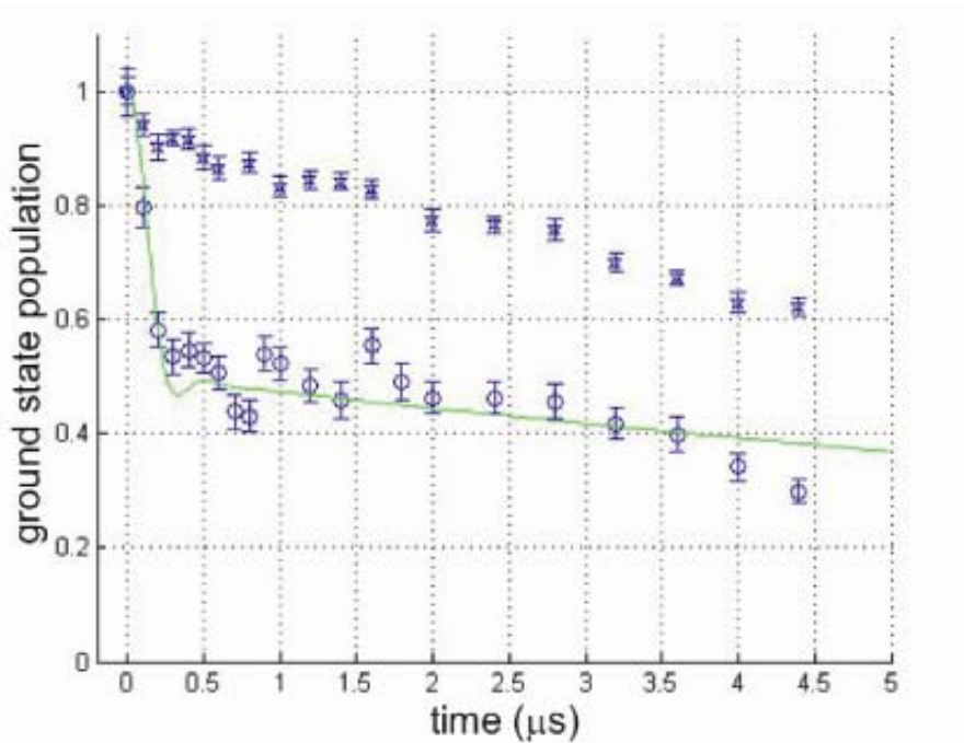
Figure 2. Time evolution of the ground state population during coherent excitation of the 28d5/2 level. The lower curve is for an average of 2 atoms in the optical trap and the upper curve is for an average of 10 atoms. The green line is a simulation result.
