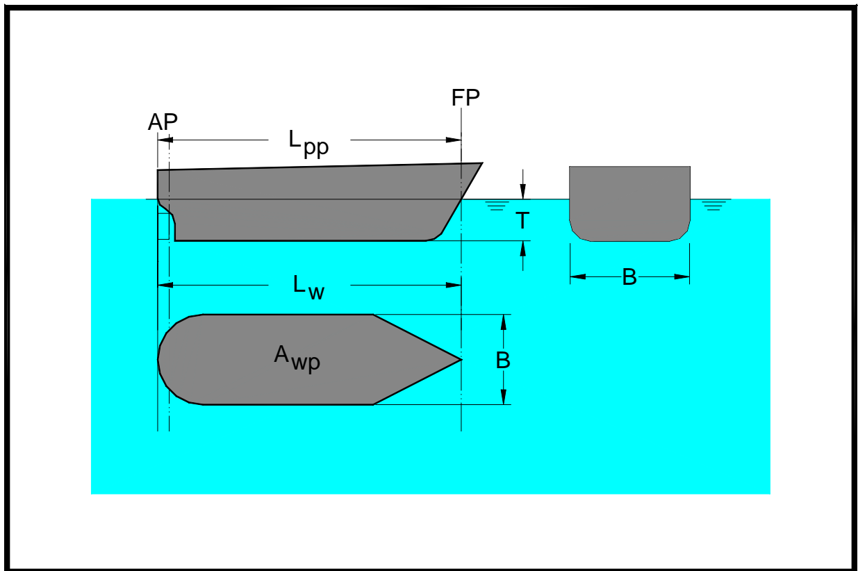
Figure 2. Ship parameters.
